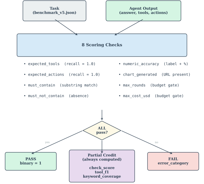
Figure 2: Scoring pipeline. Each case is evaluated by up to eight checks; binary pass requires all to pass. Partial-credit metrics (check score, tool F1, keyword coverage) are always computed.
