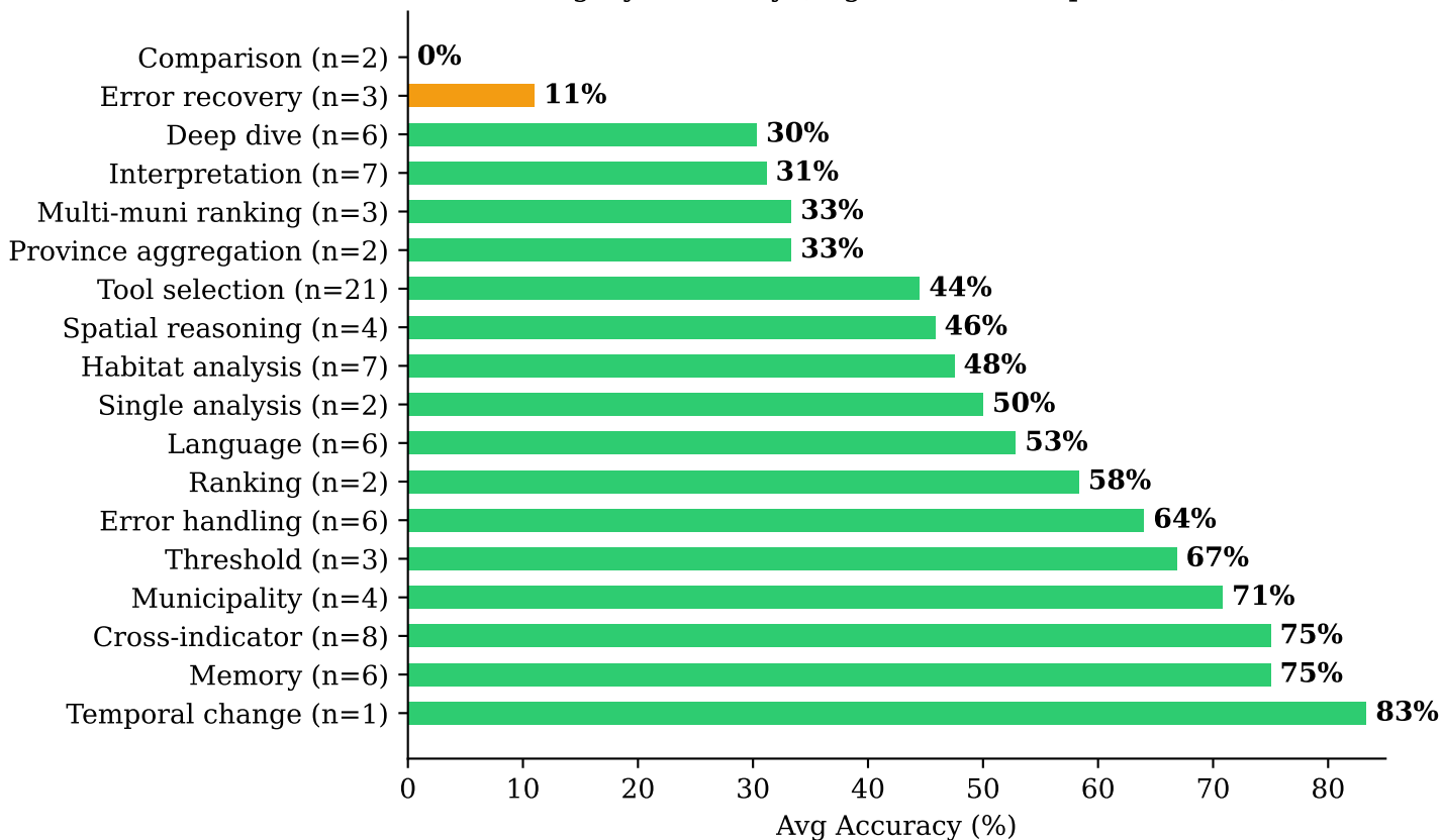
Category Difficulty (avg across 6 completed models)
