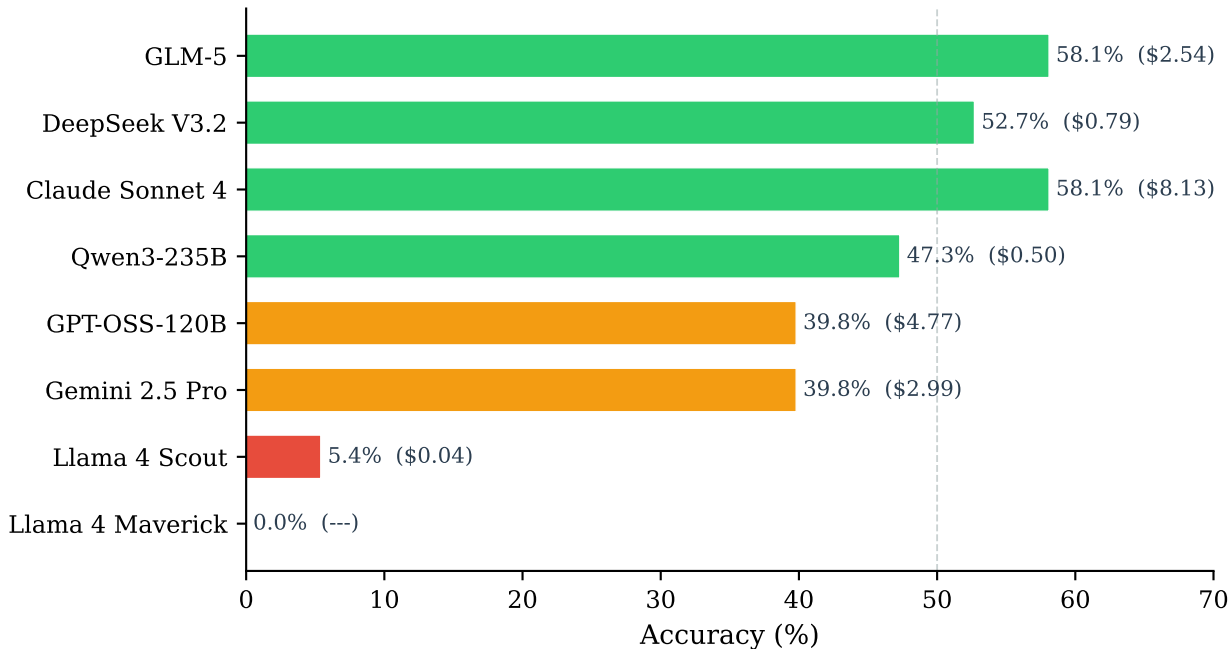
GeoAgentBench v5 — Model Accuracy (93 tasks, 8 models)
