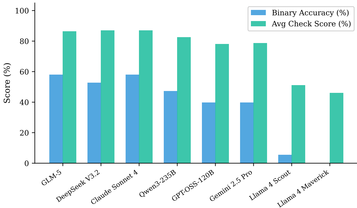
Binary Accuracy vs Partial Credit (93 tasks)
