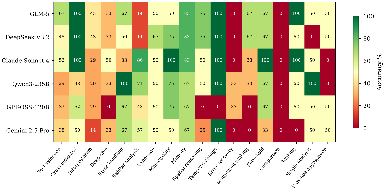
Accuracy by Category (%) — 18 categories, 6 completed models
