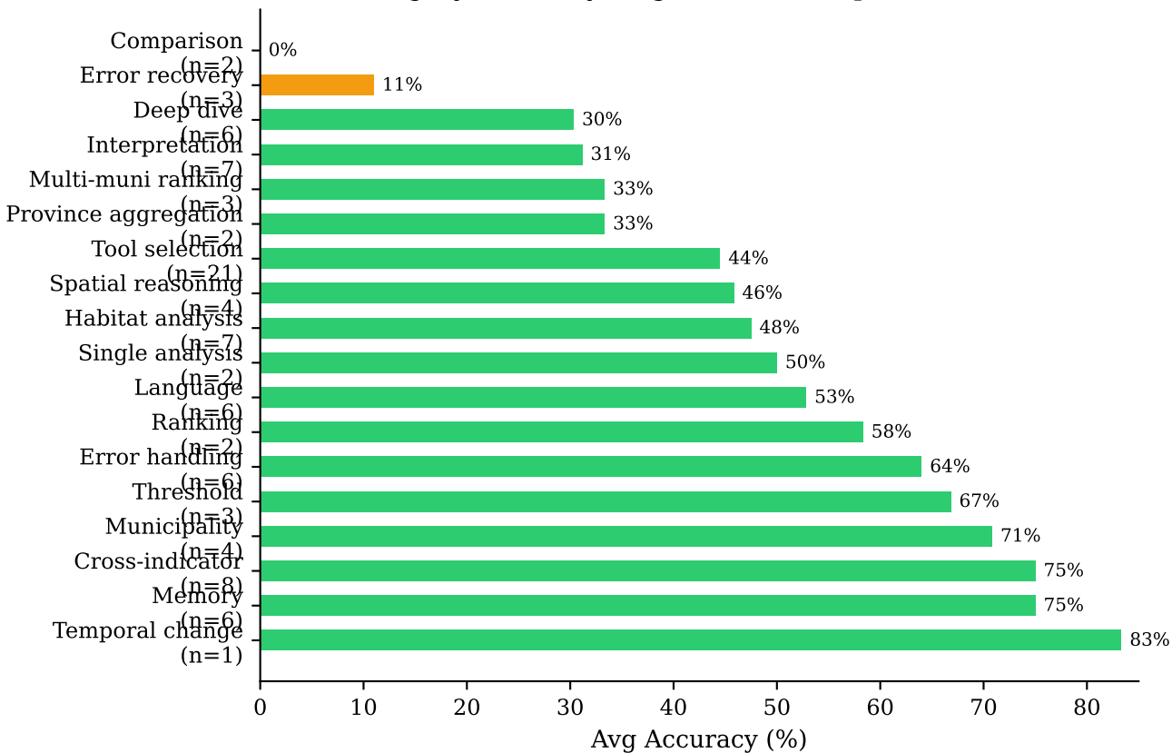
Category Difficulty (avg across 6 completed models)
