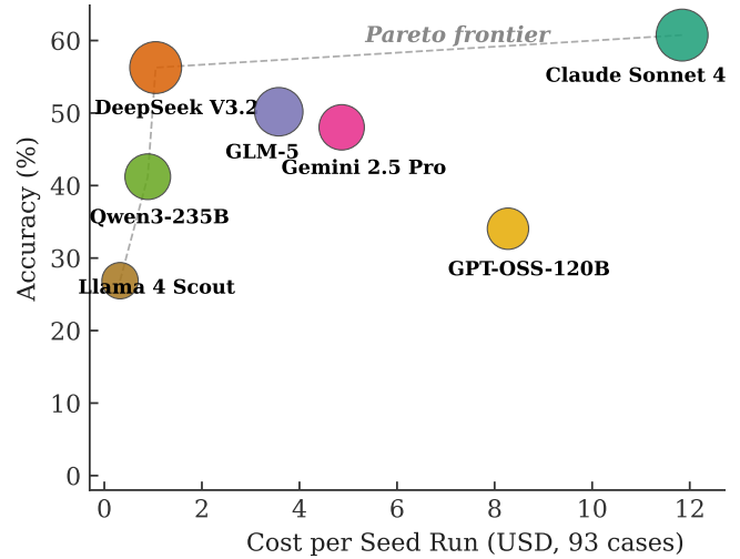
Figure 5: Cost-accuracy trade-off. Bubble size proportional to total tokens; cost is the mean per-seed run cost (93 cases). The Pareto frontier (dashed line) runs Scout → Qwen3-235B → DeepSeek V3.2 → Claude Sonnet 4: three of the four frontier models are open-weight.
