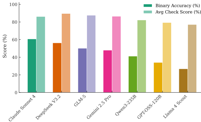
Figure 4: Binary accuracy vs partial-credit check score. The gap indicates many “miss” failures.
