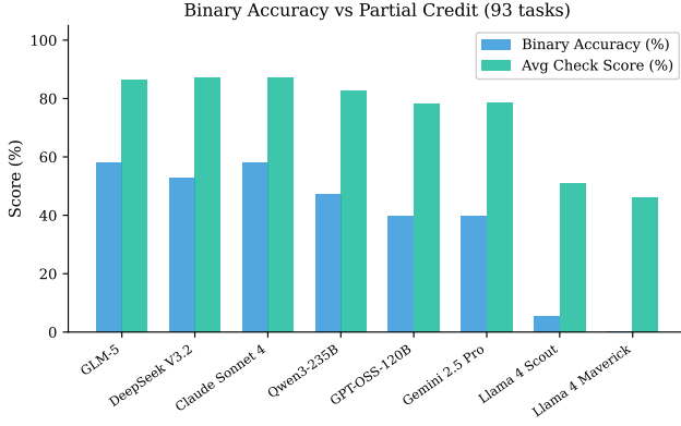
Figure 4: Binary accuracy vs partial-credit check score. The gap indicates many “near-miss” failures.
