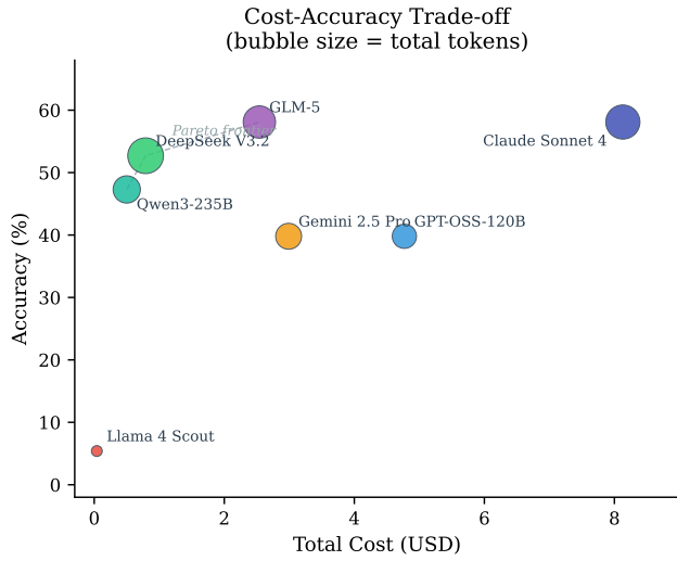
Figure 5: Cost-accuracy trade-off. Bubble size proportional to total tokens. Qwen3-235B and DeepSeek V3.2 dominate the Pareto frontier.
