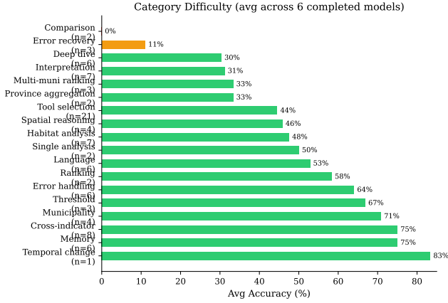
Figure 7: Universally hard categories—average accuracy across all completed models.
