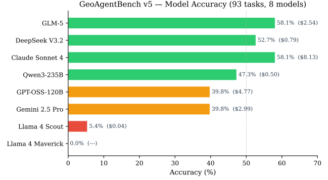
Figure 3: GeoAgentBench v5 leaderboard. Accuracy (%) with total cost in parentheses. Dashed line at 50%.
