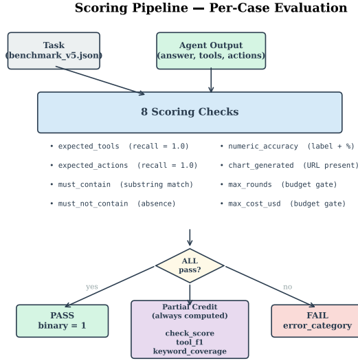
Figure 2: Scoring pipeline. Each case is evaluated by up to eight checks; binary pass requires all to pass. Partial-credit metrics (check score, tool F1, keyword coverage) are always computed.
