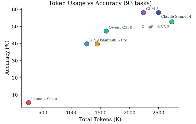
Figure 6: Token consumption vs accuracy. Token volume is a poor predictor of performance.
