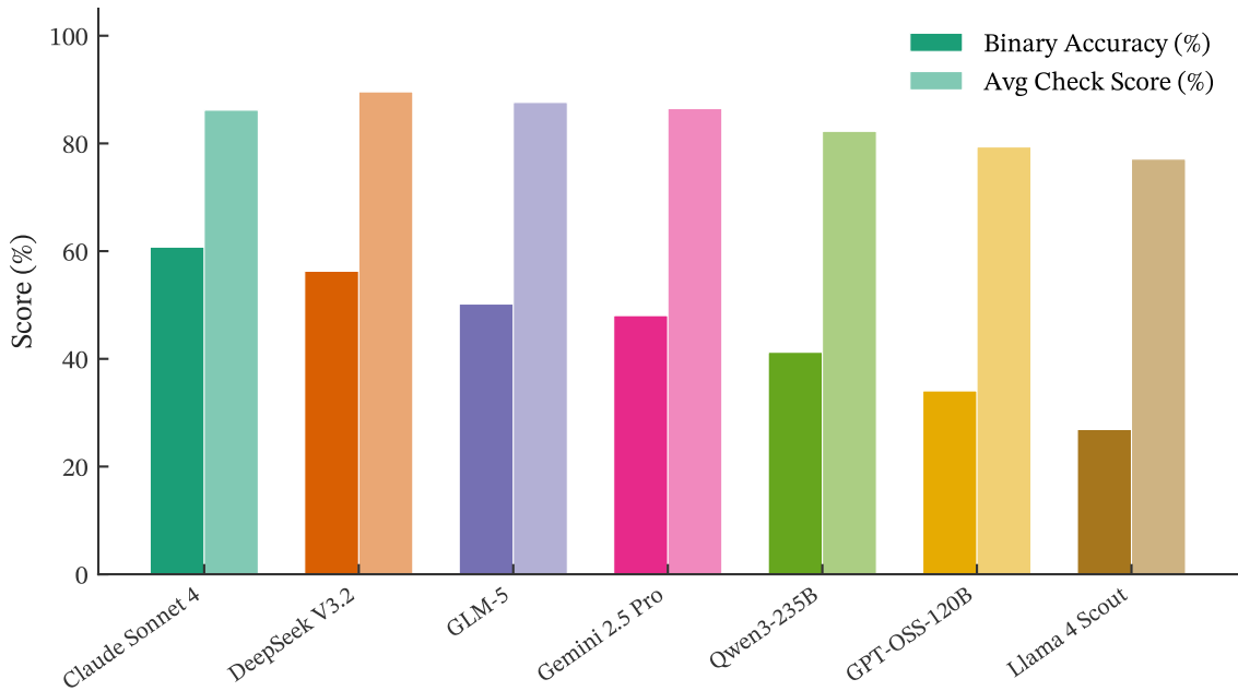
Binary Accuracy vs Partial Credit (93 tasks)
