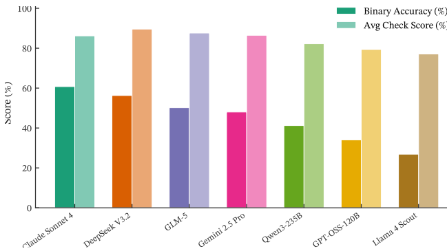
Figure 4: Binary accuracy vs partial-credit check score. The gap indicates many “near-miss” failures.
