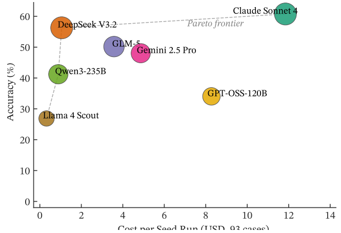
Figure 5: Cost-accuracy trade-off. Bubble size proportional to total tokens; cost is the mean per-seed run cost (93 cases). The Pareto frontier (dashed line) runs Scout → Qwen3-235B → DeepSeek V3.2 → Claude Sonnet 4: three of the four frontier models are open-weight.
