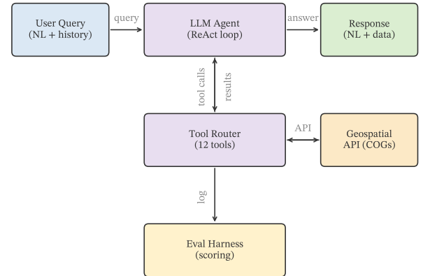
GeoNatureAgent Benchmark — System Architecture
