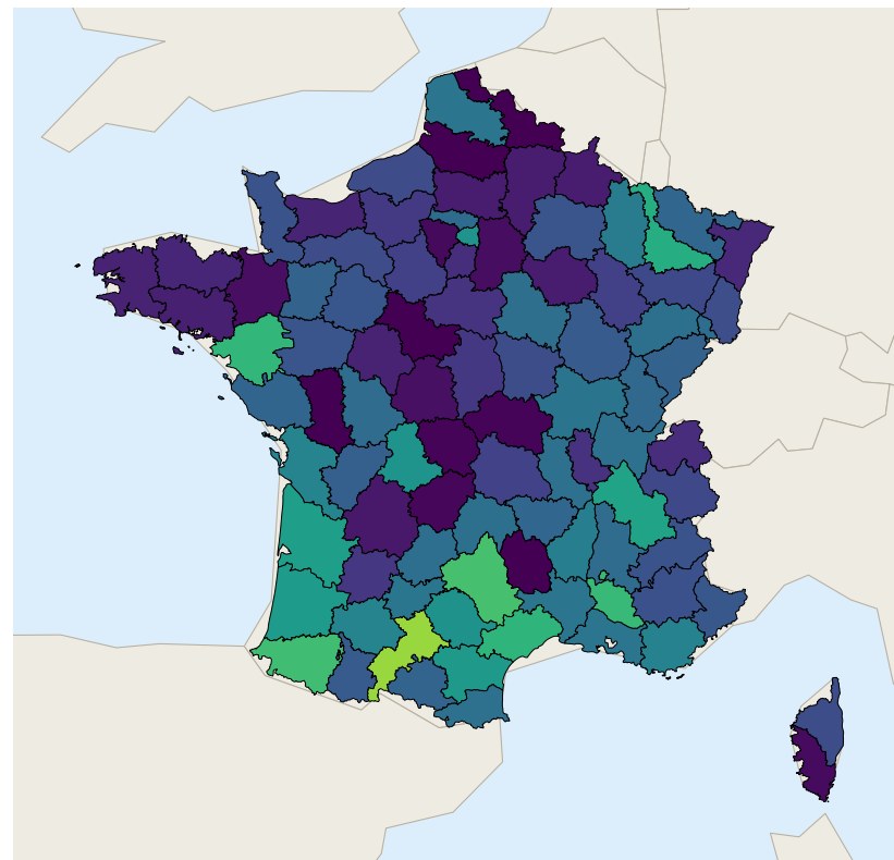
b Recall
