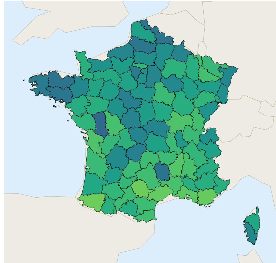
Recall
