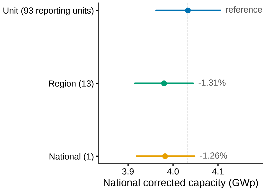
b Mean and 95% credible interval
