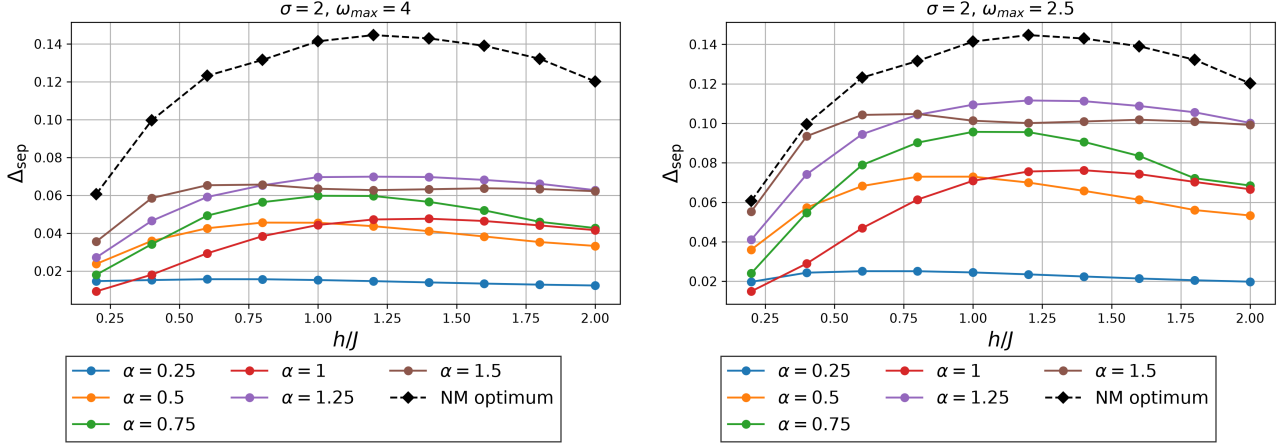
(a) Higher frequency cutoff \omega_{\text{max}} = 4 resulting in \Delta\omega = 0.4 and smaller spectral separation (b) Lower frequency cutoff \omega_{\text{max}} = 2.5 resulting in \Delta\omega = 0.25 and larger spectral separation
