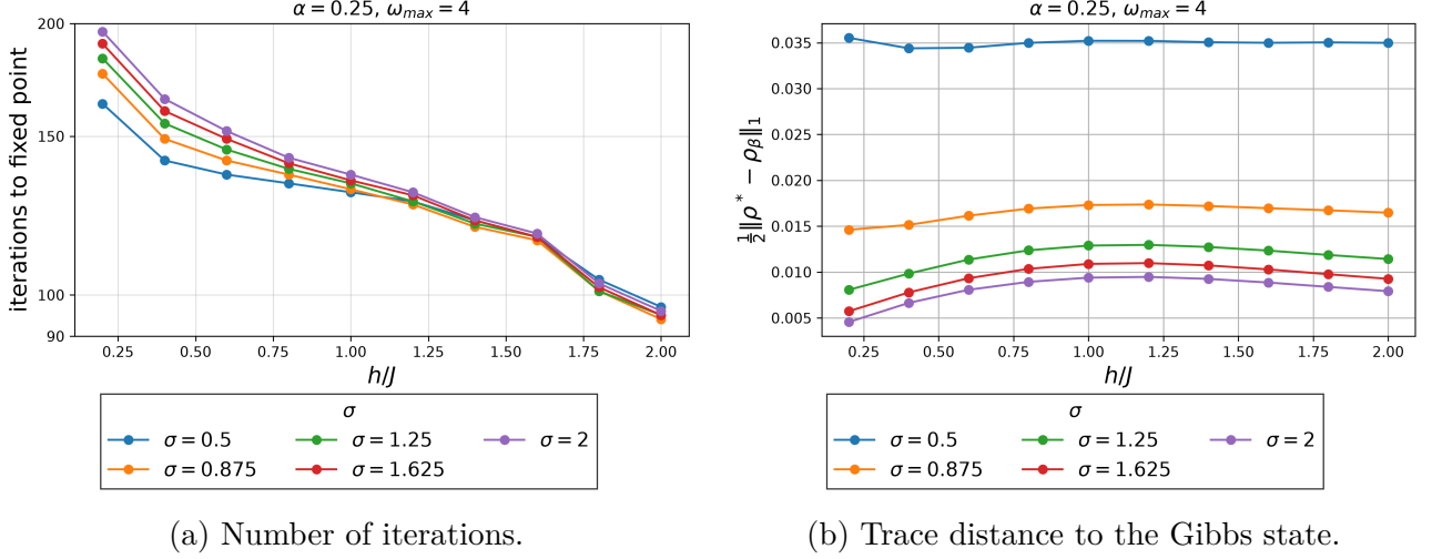
Figure 11: Number of iterations required for convergence within trace-distance \varepsilon = 0.05 to the channel fixed point and trace distance between the channel fixed point and the Gibbs state for the TFIM cooling channel with N = 4 , \alpha = 0.25 , \beta = 1 , and \omega_{\max} = 4 , for different temporal widths \sigma .
