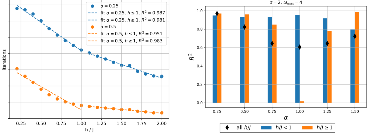
(a) Piecewise linear fits in the semilog plot for h/J \leq 1 and h/J \geq 1 . (b) Fit quality ( R^2 ) of the semilog regressions in the h/J \leq 1 and h/J \geq 1 regions.
