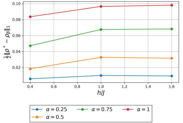
(b) N = 6 spins.
