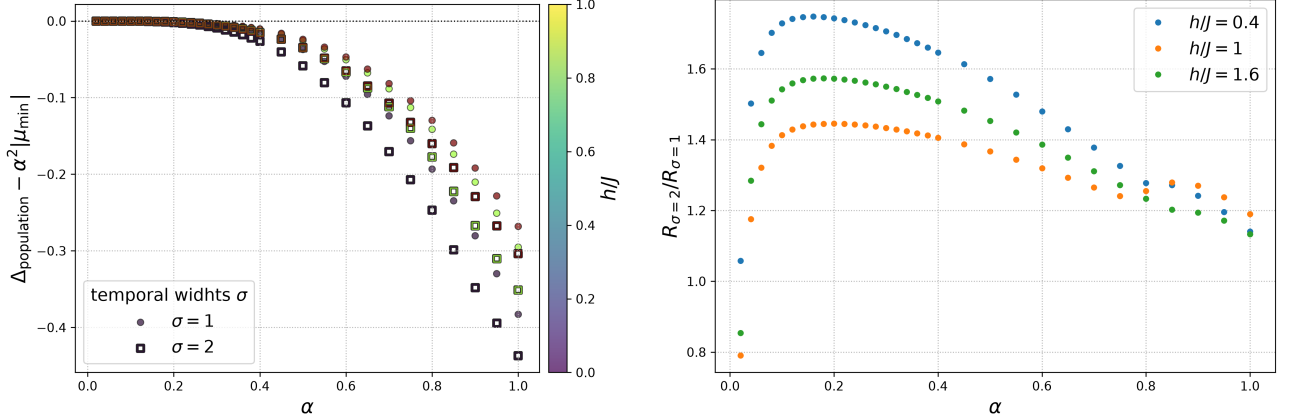
(a) Parameter dependence of signed residuals of the generator gap-estimate for \sigma = 2 and \sigma = 1 . (b) Parameter dependence of residuals ratio from generator gap-estimate for \sigma = 2 and \sigma = 1 .
