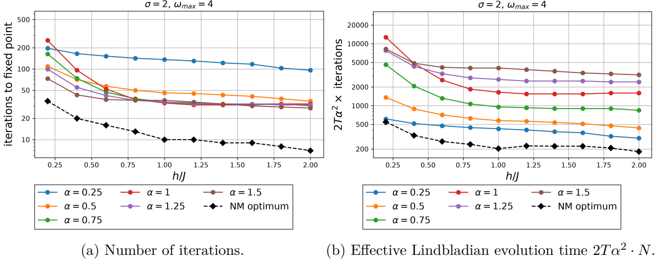
Figure 3: Convergence within trace-distance \varepsilon = 0.05 to channel fixed-point for the TFIM with N = 4 cooling channels, for various values of the coupling-strength \alpha . NM refers to parameter configurations obtained using the gradient free Nelder-Mead optimizer.
