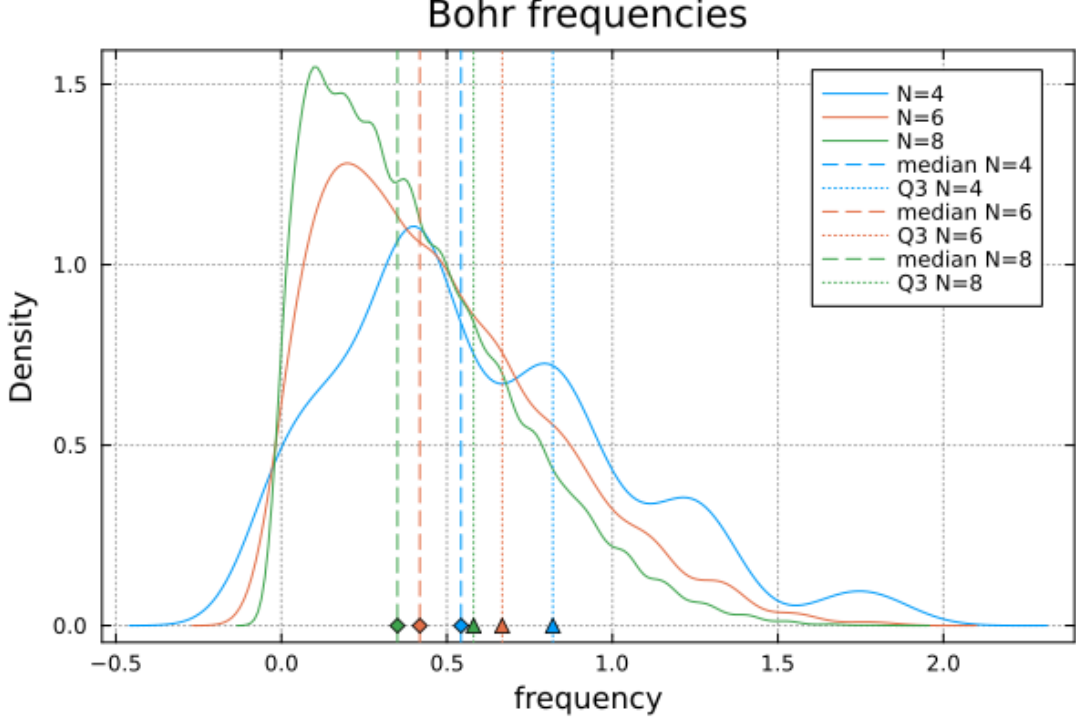
Figure 1: TFIM for h = 1.2 , J = 1 and normalization factor N\sqrt{J^2 + h^2} .
