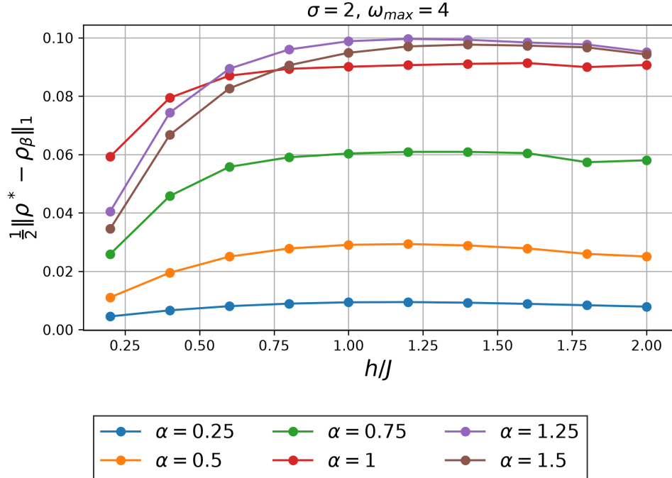
Figure 5: Trace distance between the channel fixed point and the Gibbs state for the TFIM cooling channel with N = 4, \beta = 1, \sigma = 2 , and \omega_{\max} = 4 , for different coupling strengths \alpha .
