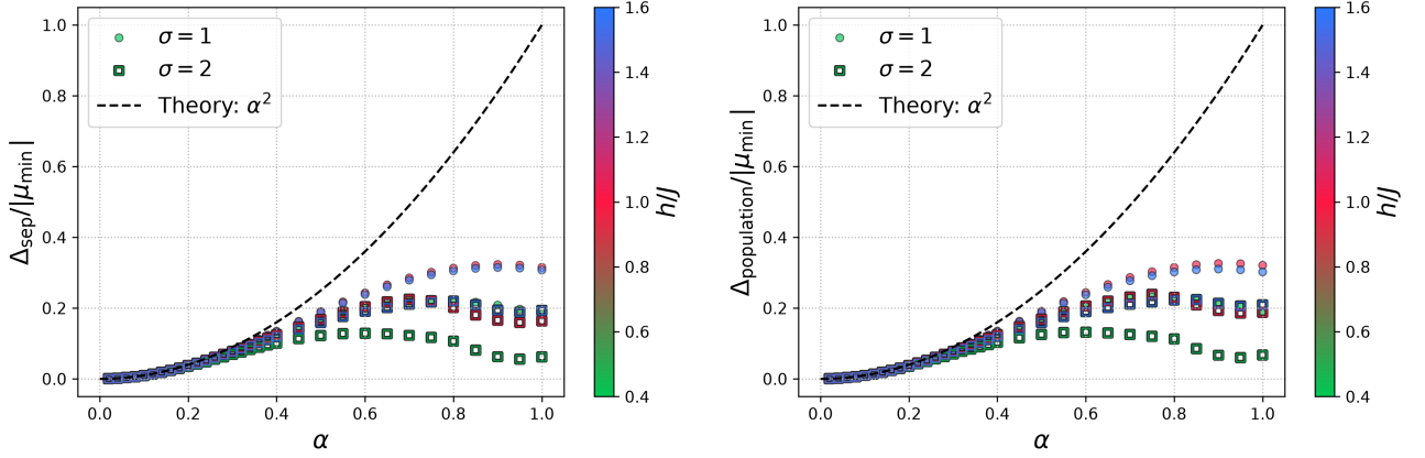
(a) Dependence of spectral gap of full channel \mathcal{E} . (b) Dependence of spectral gap of channel restricted to classical mixtures of \rho = \sum_i p_i |i\rangle \langle i| .
