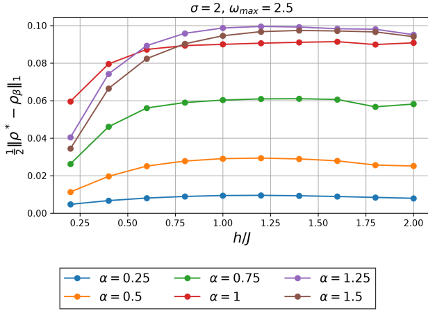
(a) N = 4 spins.
