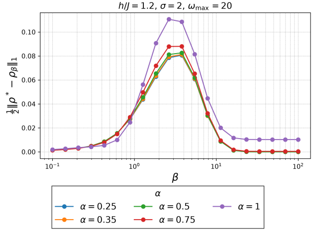
(b) Trace distance to the Gibbs state.
