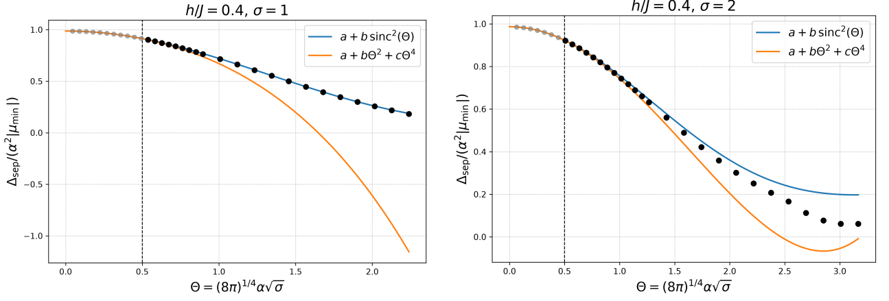
(a) Approximation of the full channel spectral gap by the generator gap. (b) Approximation of the population-sector spectral gap by the generator gap.
