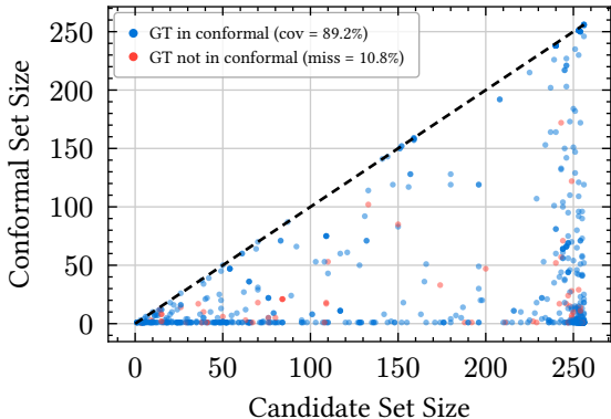
Conformal Set Size vs Candidate Set Size
