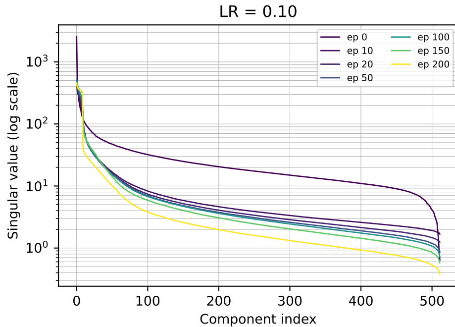
Singular value spectrum at selected epochs
