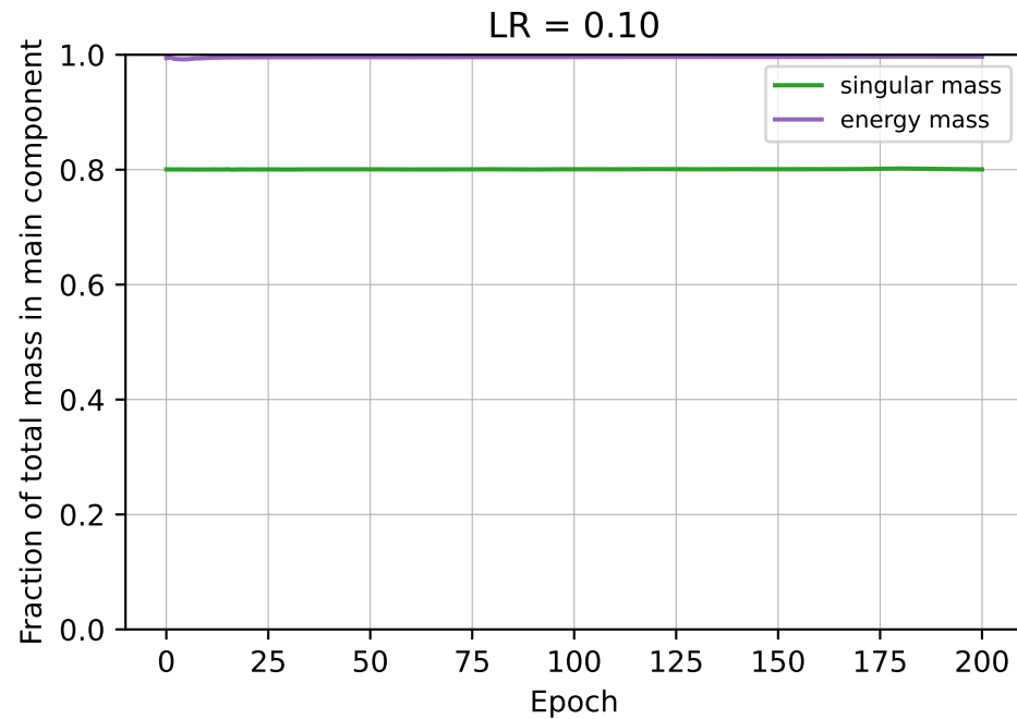
Main spectral mass and energy mass over training
