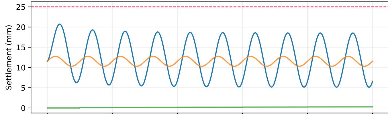
Bridge-abutment retrofit
