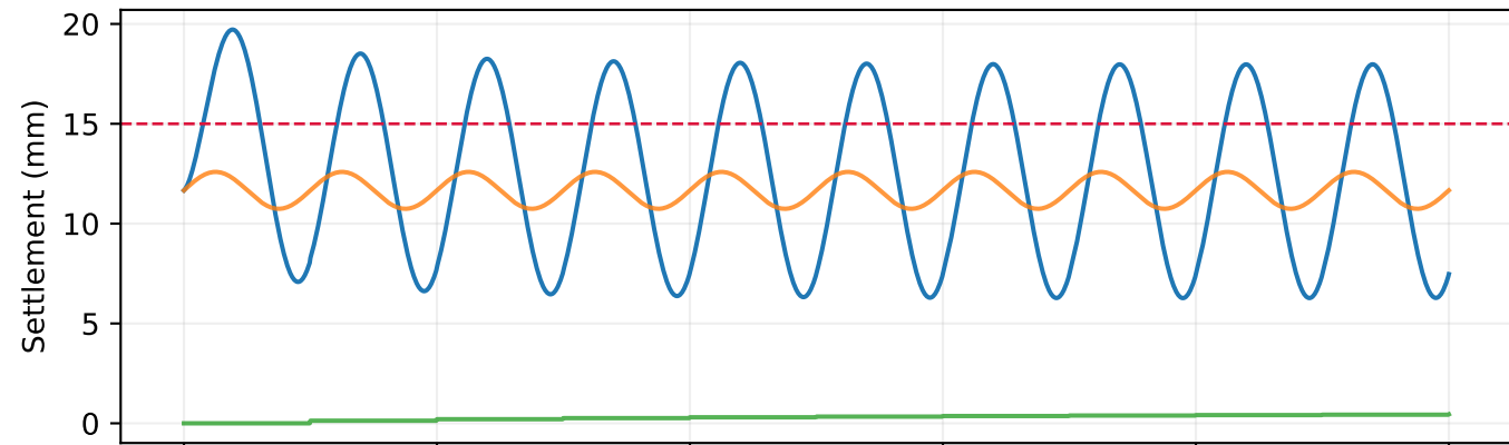
Equipment-supported mat
