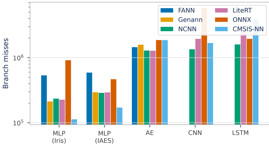
Branch Misses (total per 1000 inferences)
