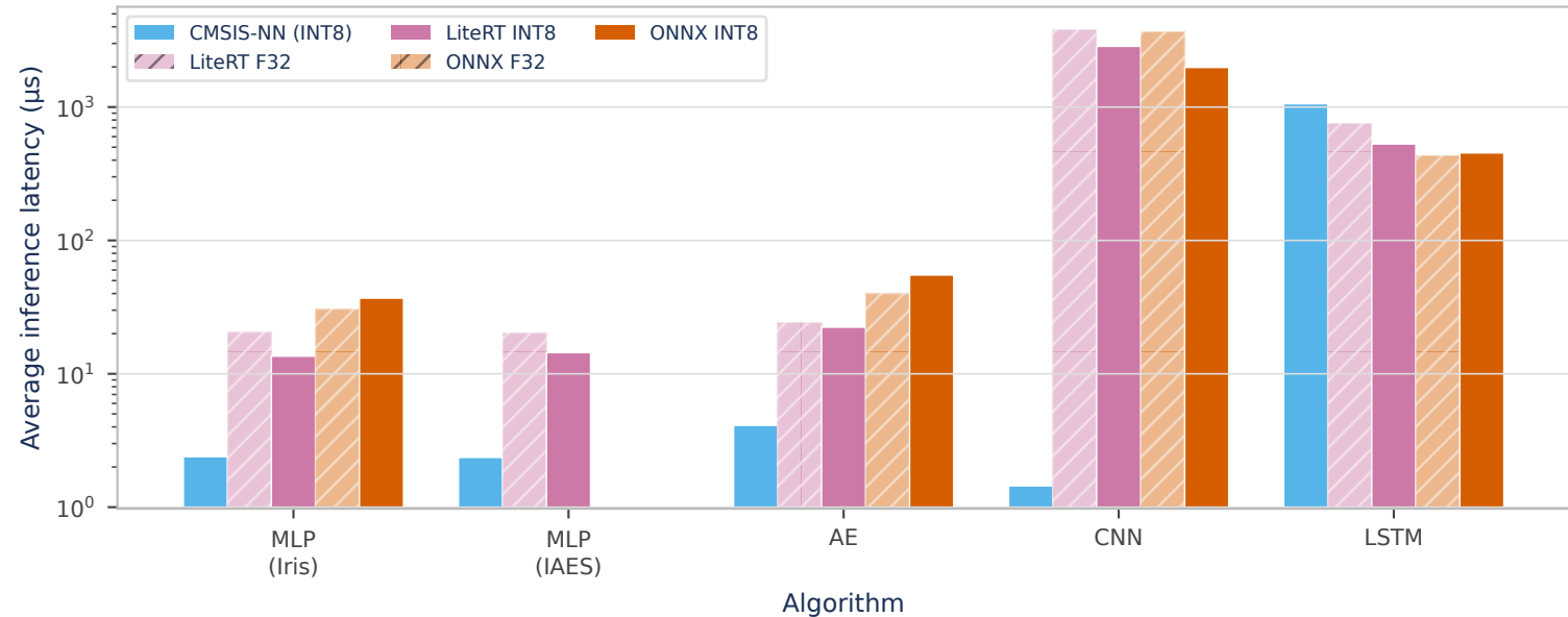
INT8 vs F32 inference latency comparison
