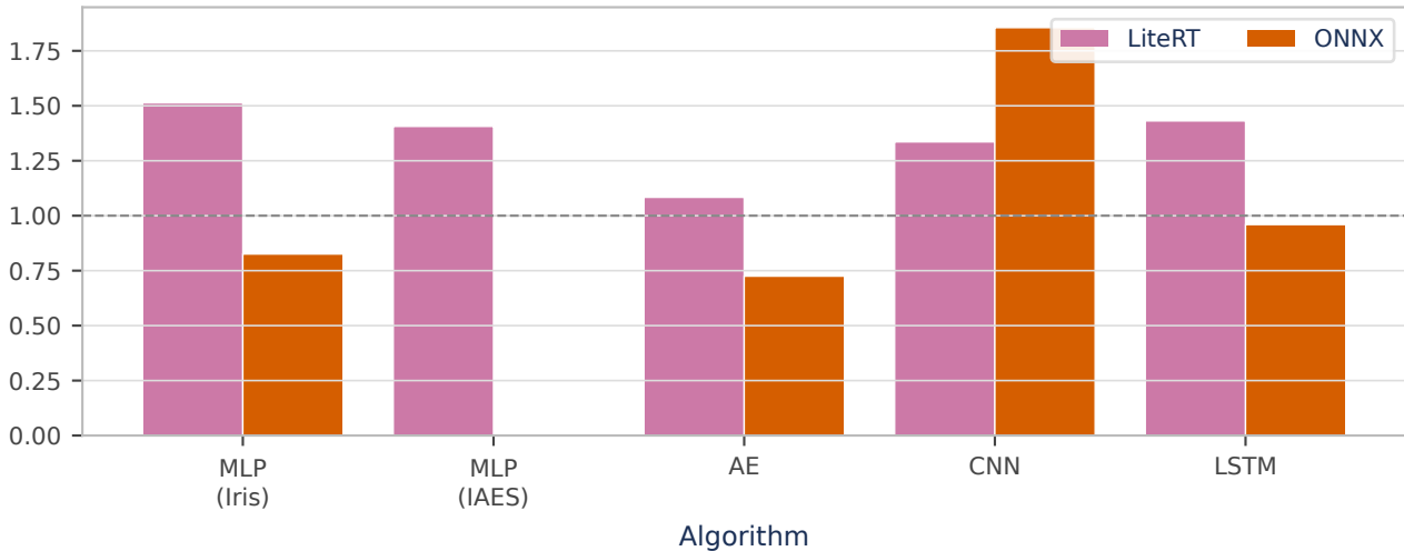
INT8 speedup over F32 per framework
