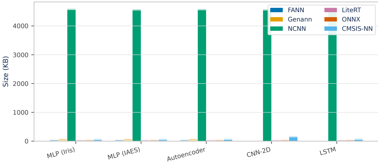
Static memory footprint of executables (solid = .text, transparent = .bss)
