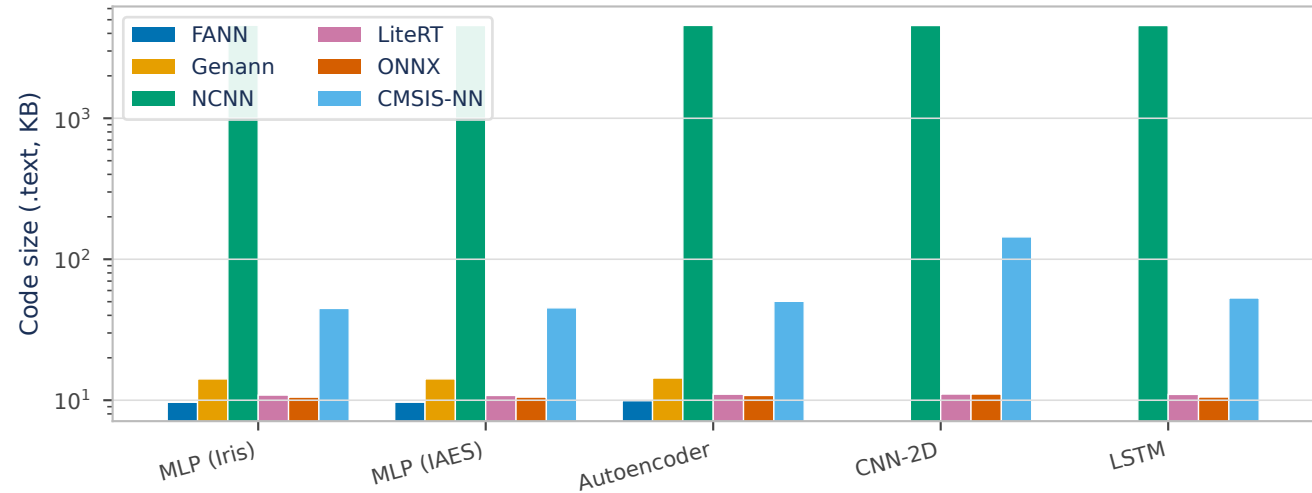
Compiled code size per framework and algorithm
