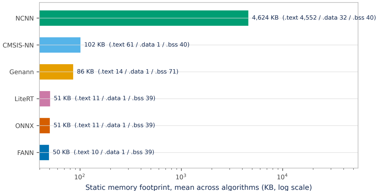
Executable memory footprint by framework
