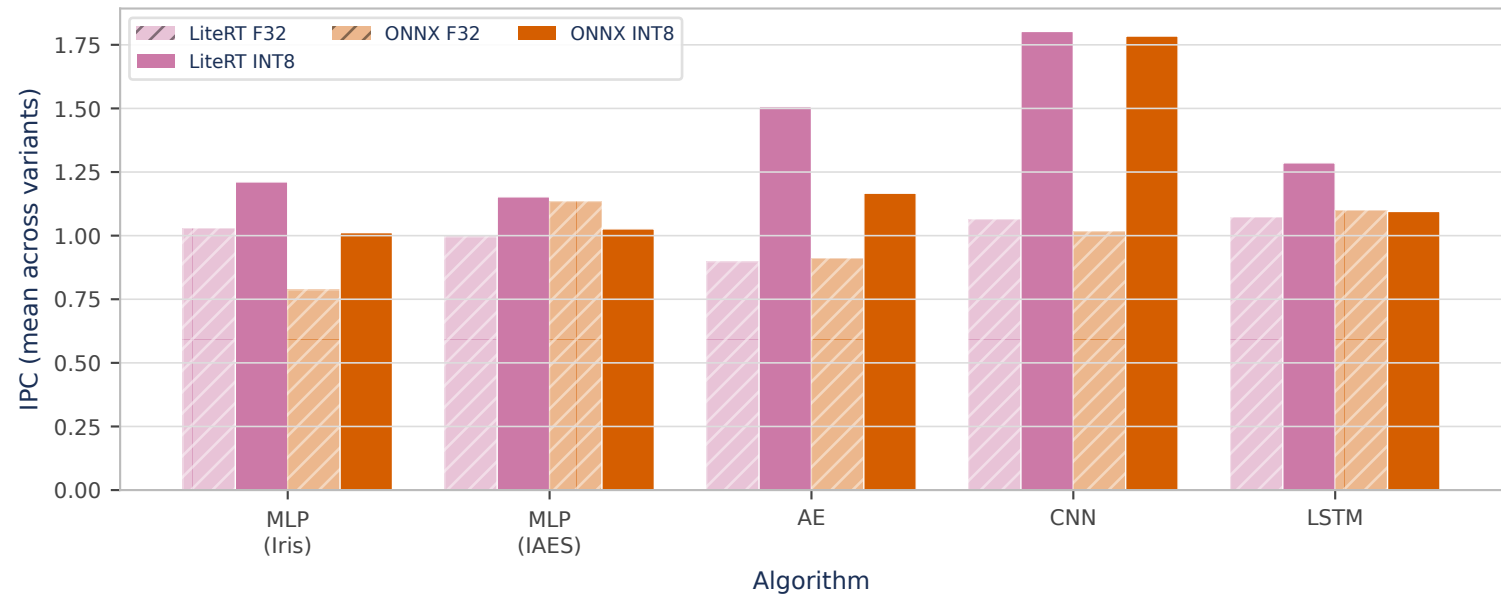
IPC comparison — F32 vs INT8
