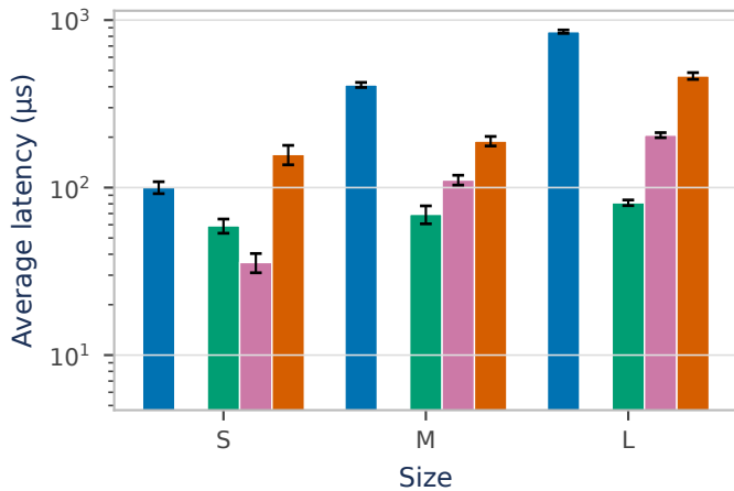
ReLU
