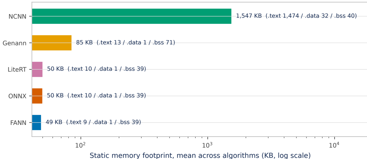
Executable memory footprint by framework (RISC-V)
