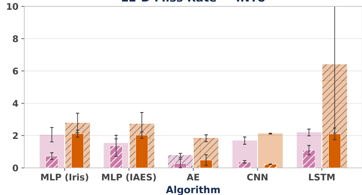
L1-D Miss Rate — INT8
