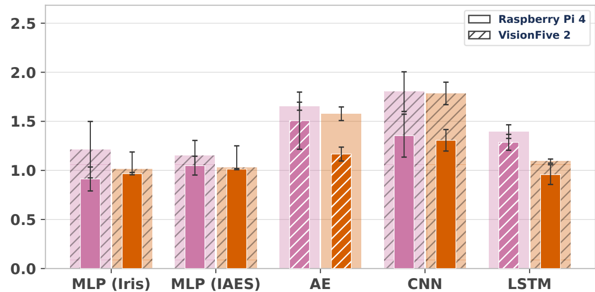
L1-D Miss Rate — INT8
