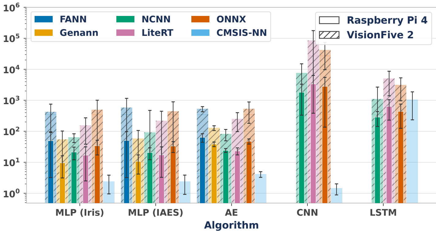
Avg. inference latency ( \mu\text{s} , log scale)
