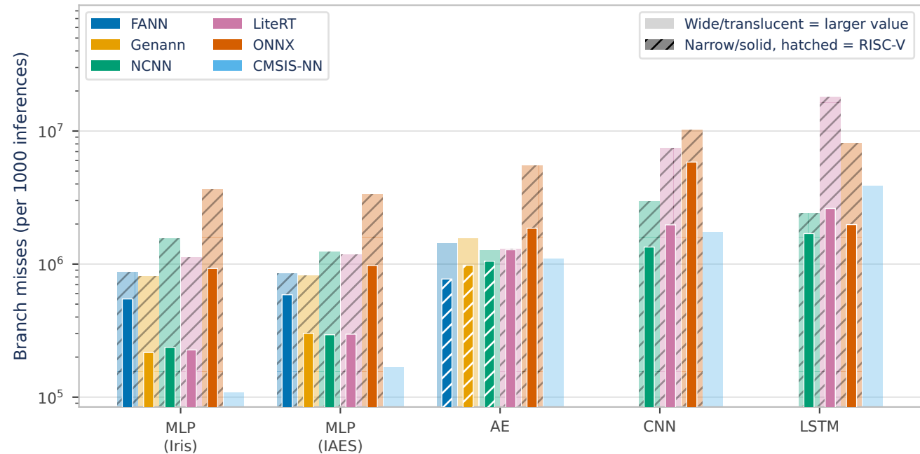
Branch misses, RPi vs RISC-V overlaid
