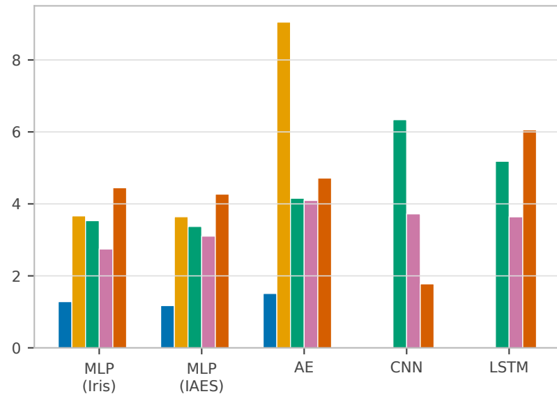
L1-D Miss Rate — VisionFive 2 (RISC-V)
