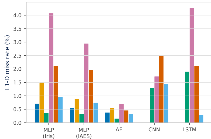
L1-D Miss Rate — Raspberry Pi 4
