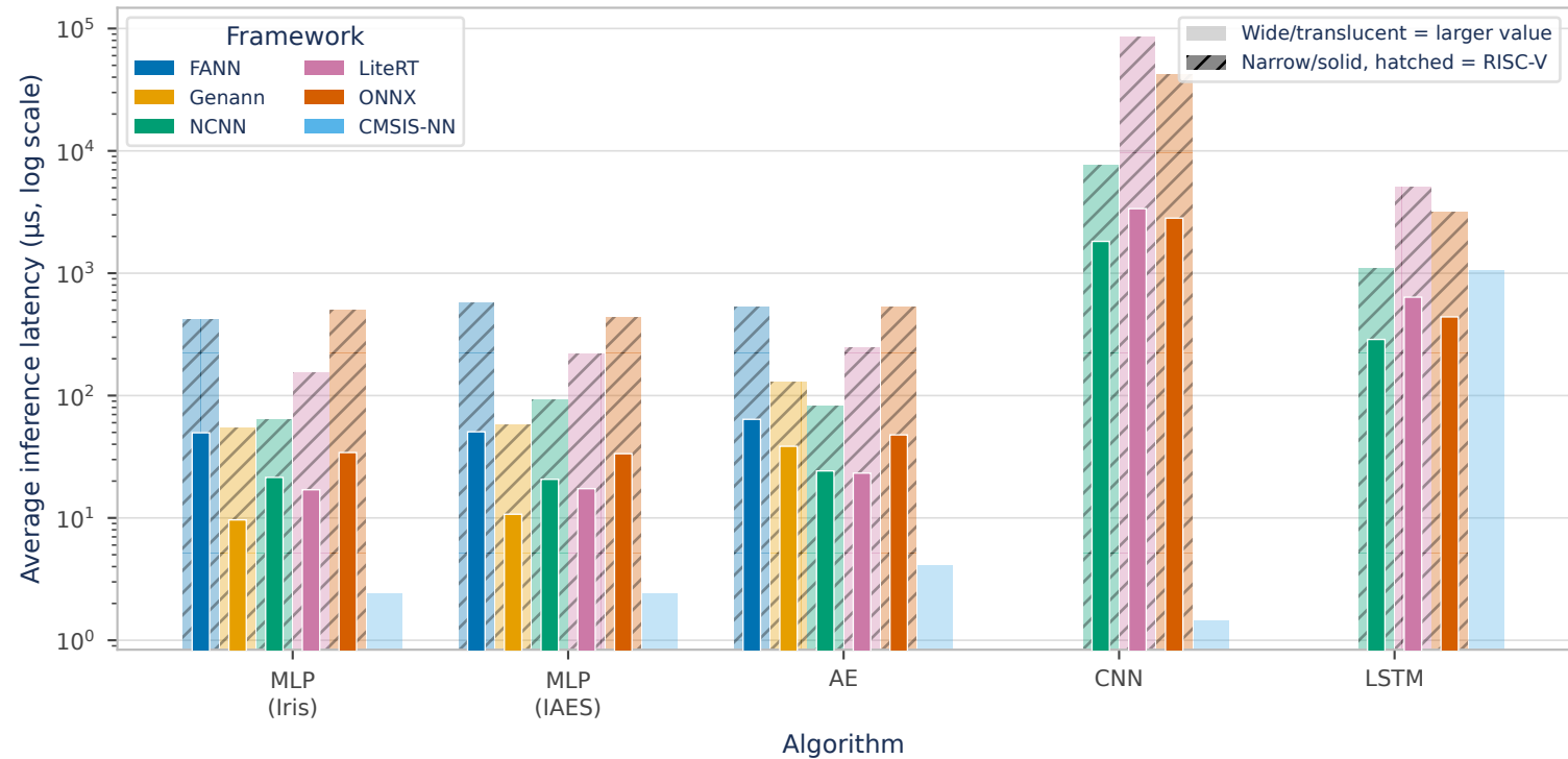
Inference latency, RPi vs RISC-V overlaid
