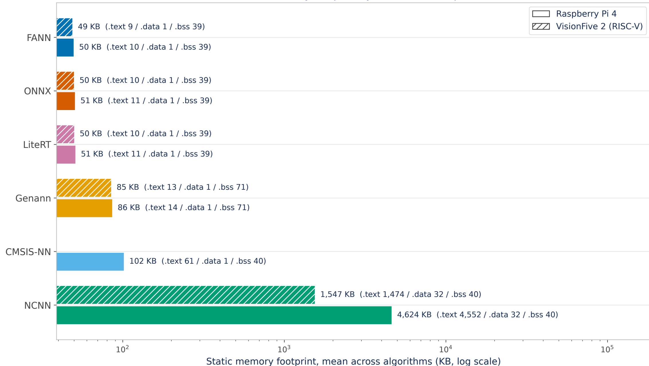
Executable memory footprint by framework and platform
