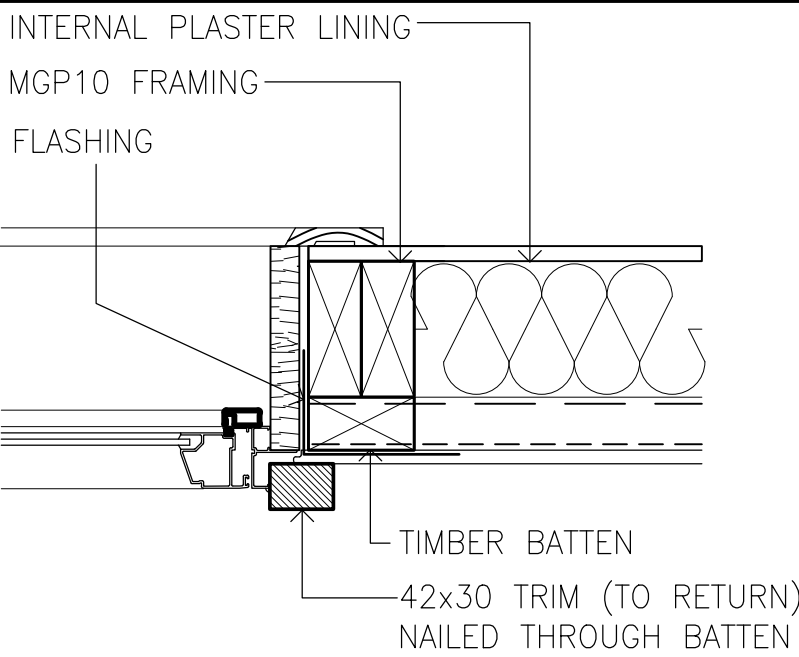
ALUMINIUM WINDOW: PLAN
