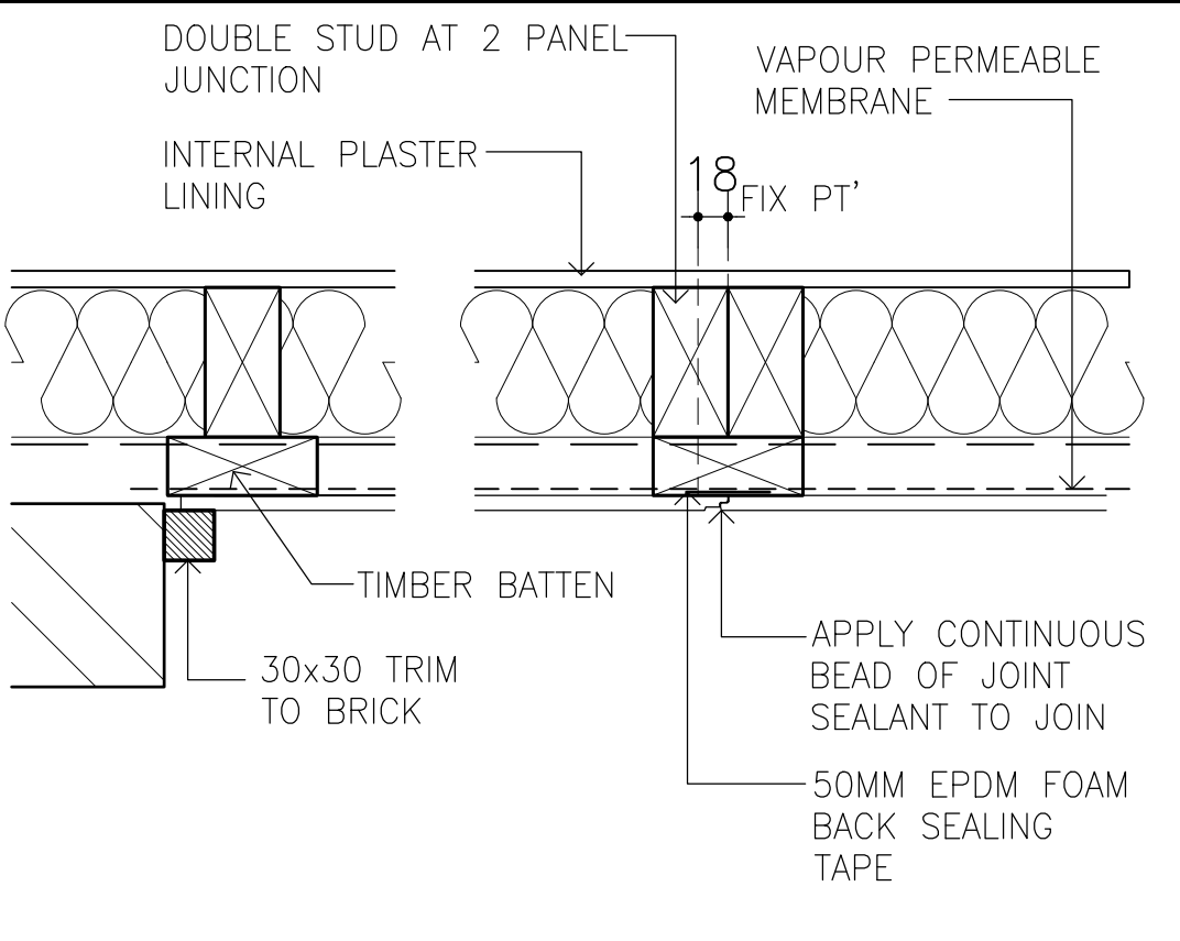
HORIZONTAL JOINT & EASYLAP TO BRICK
