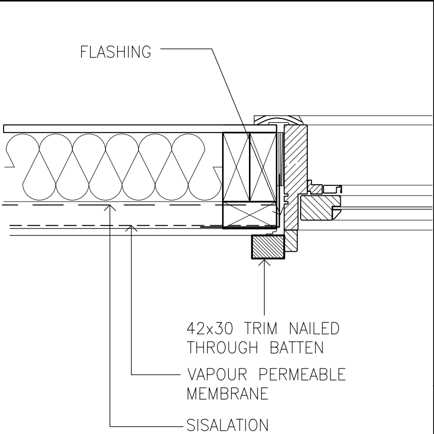
TIMBER WINDOW: PLAN
