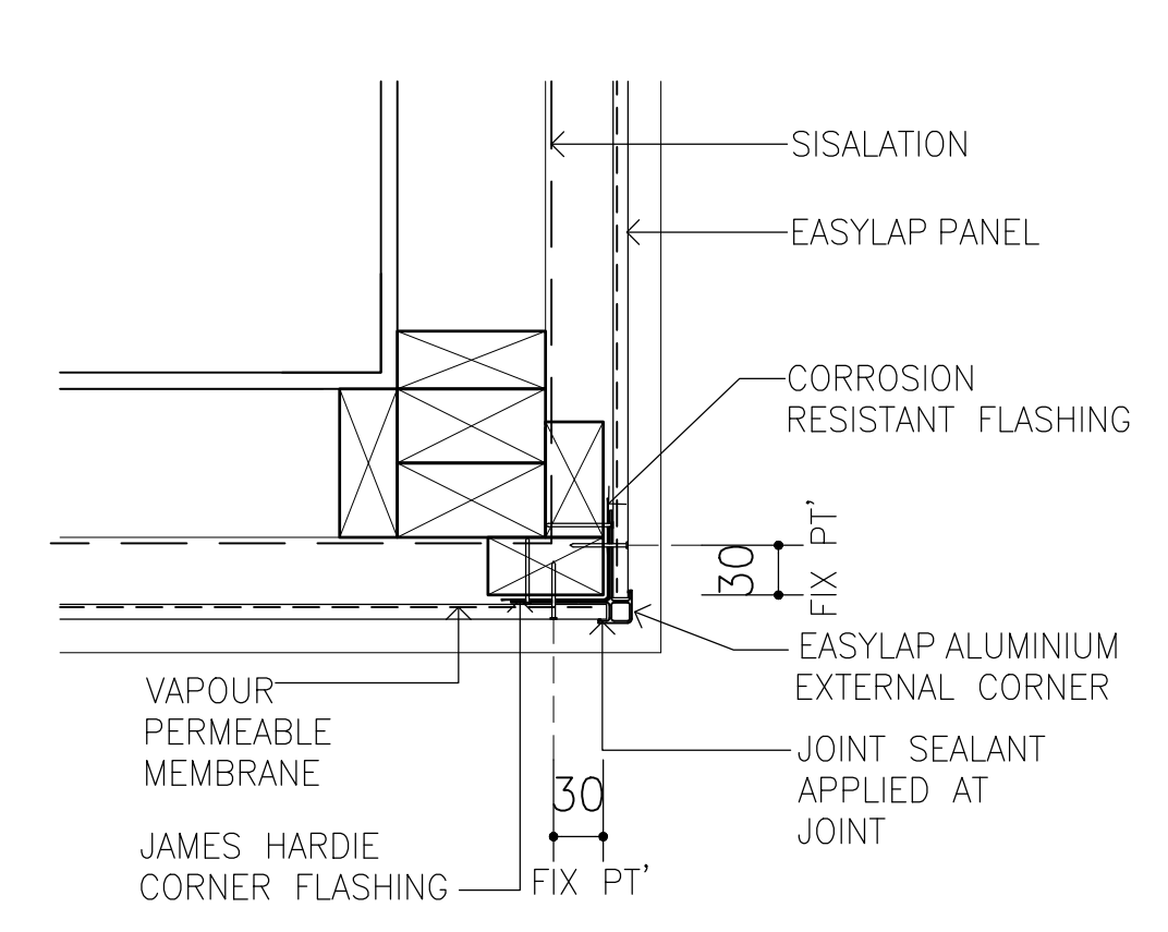
EXTERNAL BOX CORNER
