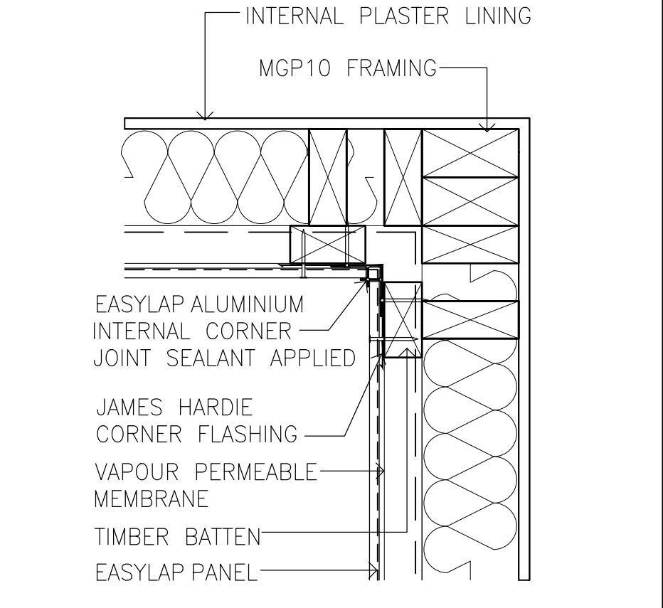
INTERNAL BOX CORNER
