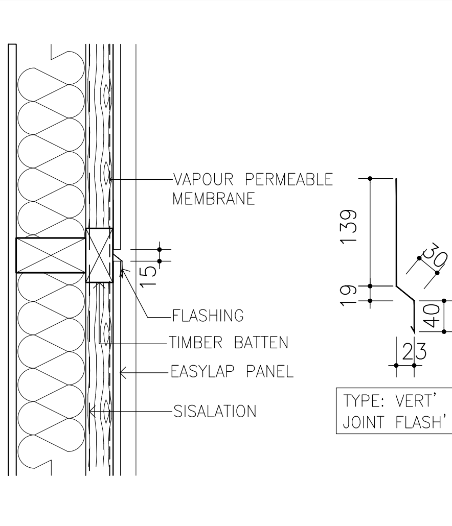
VERTICAL SECTION
