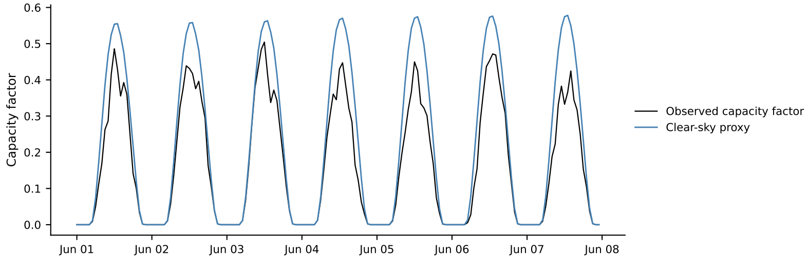
Solar production and clear-sky proxy
