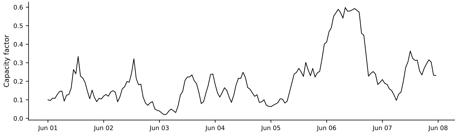
Wind capacity factor
