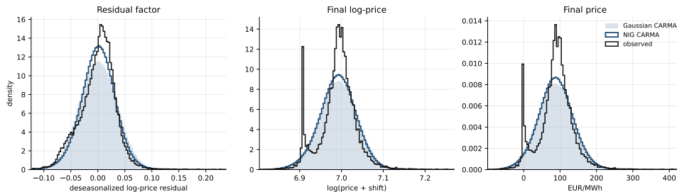
Figure B.1: Distribution checks for the German price marginal model at the residual factor, shifted log-price, and EUR/MWh price levels.
