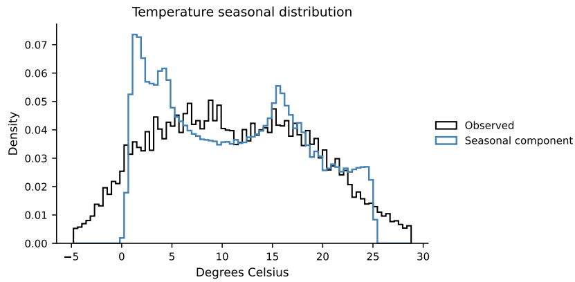
Figure A.7: Marginal distribution of observed temperature and of the fitted deterministic seasonal component over the 2023–2025 calibration sample.
