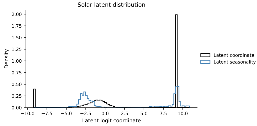
Figure A.11: Marginal distribution of the solar latent coordinate and of its fitted deterministic seasonal component over the calibration sample.
