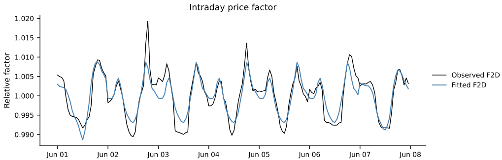
Figure A.2: Observed and fitted intraday price factor over the common appendix week. The observed factor is the shifted log-price divided by its daily mean.
