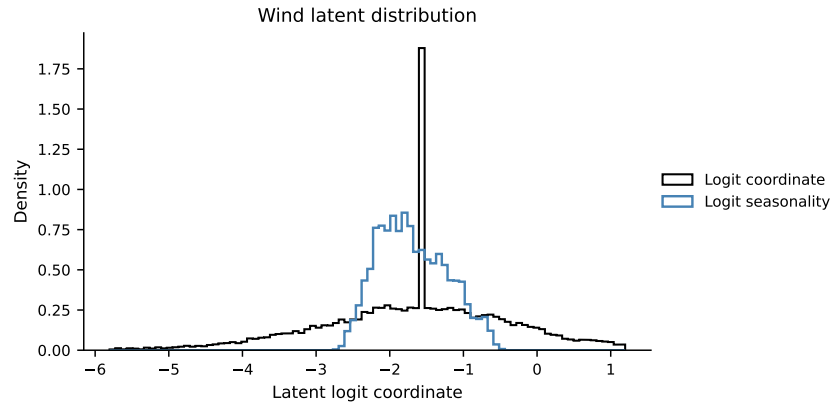
Figure A.15: Marginal distribution of the wind latent logit coordinate and of its fitted deterministic seasonal component over the calibration sample.
