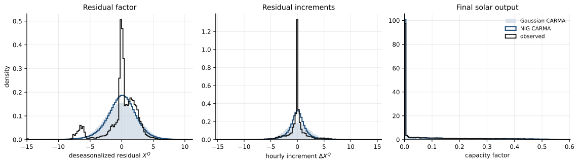
Figure B.3: Distribution checks for the German solar marginal model at the deseasonalized latent residual, hourly residual-increment, and physical capacity-factor levels.
