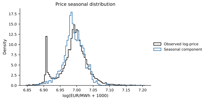
Figure A.5: Marginal distribution of the shifted log-price and of its fitted deterministic seasonal component over the 2023–2025 calibration sample.
