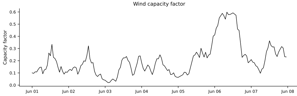
Figure A.12: Observed wind capacity factor over the common appendix week.
