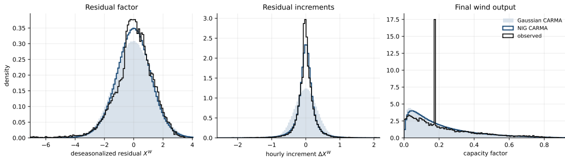
Figure B.4: Distribution checks for the German wind marginal model at the deseasonalized logit residual, hourly residual-increment, and physical capacity-factor levels.
