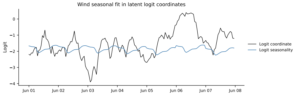
Figure A.13: Wind seasonal fit in the latent logit coordinate over the common appendix week. This is the coordinate in which the deterministic seasonality is estimated.
