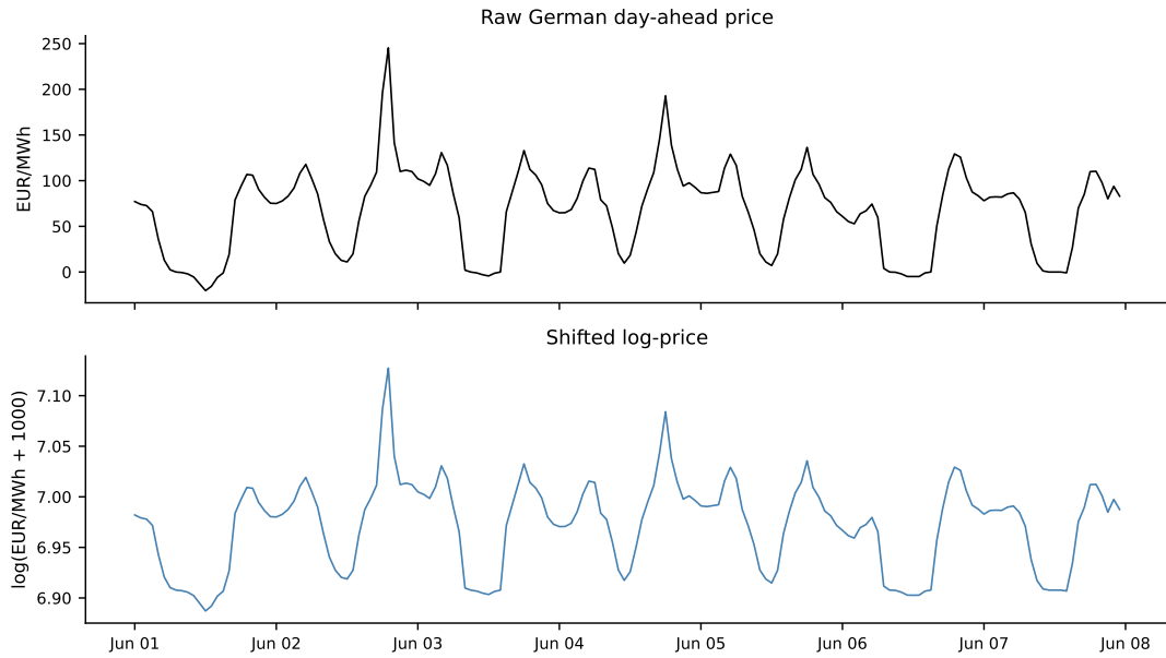
Figure A.1: German day-ahead price and shifted log-price over the common appendix week. The shift makes the logarithmic coordinate well-defined when hourly prices are negative.
