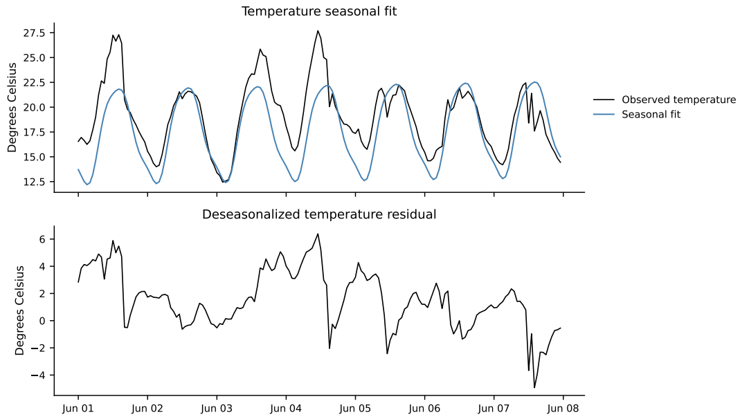
Figure A.6: Temperature seasonal fit and resulting deseasonalized residual over the common appendix week.
