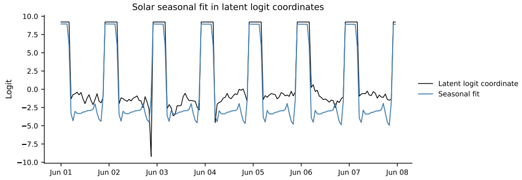
Figure A.9: Solar seasonal fit in the latent logit coordinate over the common appendix week. This is the coordinate in which the deterministic seasonality is estimated.
