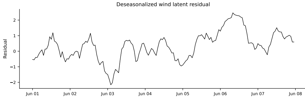
Figure A.14: Deseasonalized wind residual in the latent logit coordinate over the common appendix week. This residual is the stochastic component calibrated with a CARMA model.
