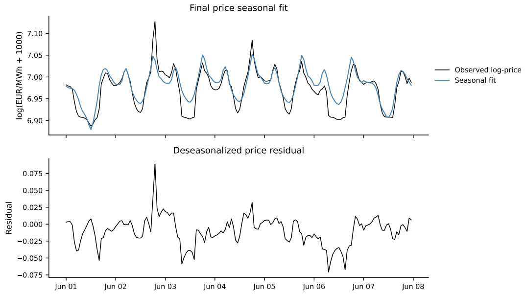
Figure A.4: Final deterministic price seasonality and resulting deseasonalized log-price residual over the common appendix week.
