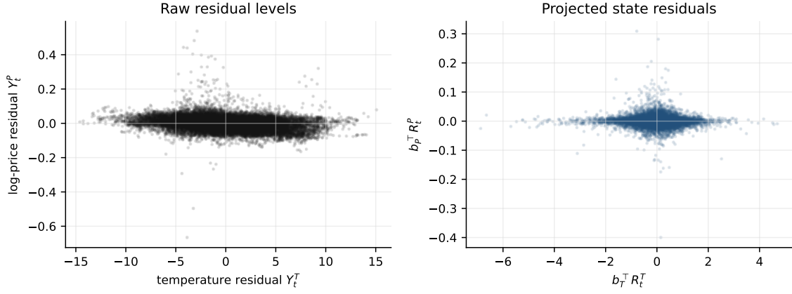
Figure C.1: Temperature–price residual scatter plots. The first panel uses raw deseasonalized residual levels. The second panel uses the projected state-space residuals entering the covariance-based coupling estimator.
