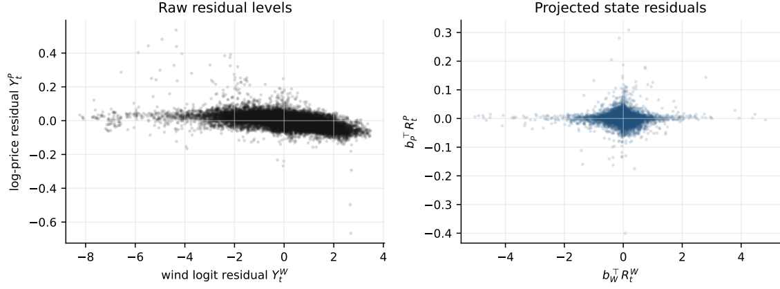
Figure C.3: Wind–price residual scatter plots. The first panel uses wind logit residual levels and the second panel uses the corresponding projected CARMA state-space residuals.
