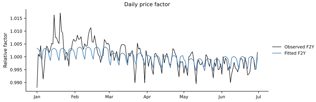
Figure A.3: Observed and fitted daily price factor over the first semester of 2025. The observed factor is the daily mean shifted log-price divided by its yearly mean.
