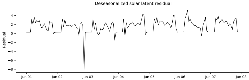
Figure A.10: Deseasonalized solar residual in the latent logit coordinate over the common appendix week. This residual is the stochastic component calibrated with a CARMA model.
