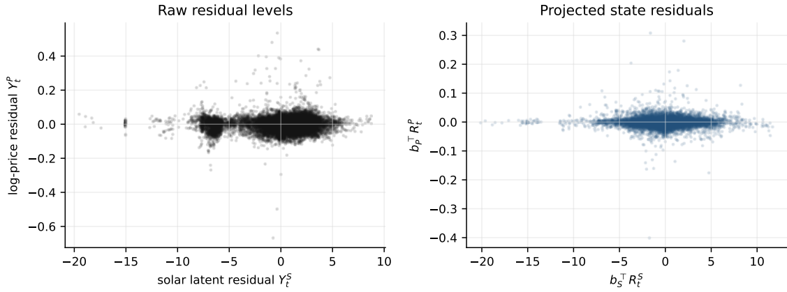
Figure C.2: Solar–price residual scatter plots. The raw residual is the solar latent shortfall coordinate, while the projected residual is obtained from the calibrated CARMA state-space filter.
