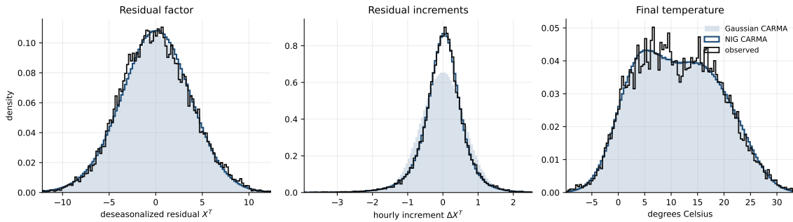
Figure B.2: Distribution checks for the German temperature marginal model at the deseasonalized residual, hourly residual-increment, and physical temperature levels.
