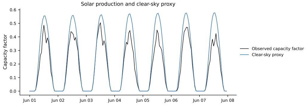
Figure A.8: Observed solar capacity factor and clear-sky proxy over the common appendix week. The clear-sky proxy is the deterministic envelope used before constructing the latent logit coordinate.
