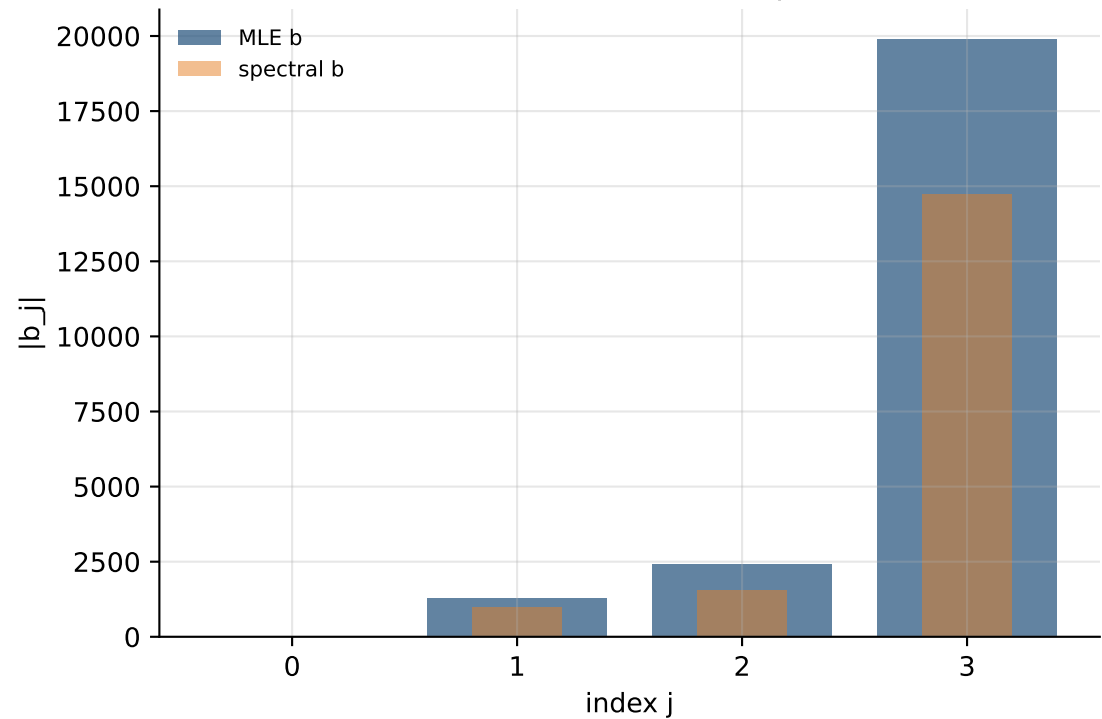
MA coefficients: MLE vs spectral
