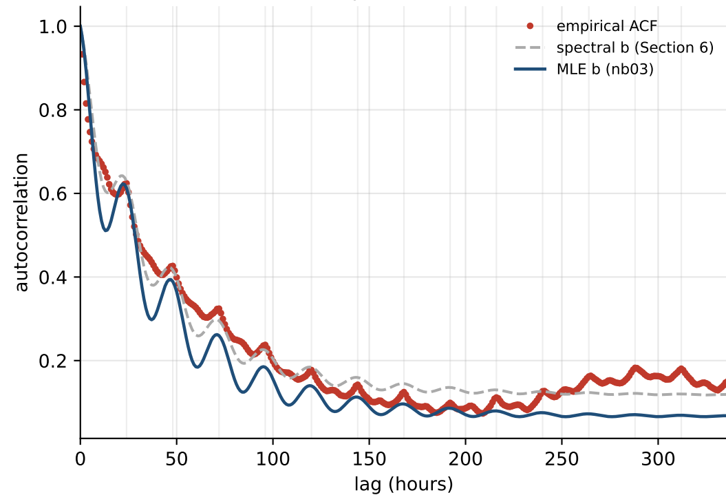
ACF fit: spectral b vs MLE b
