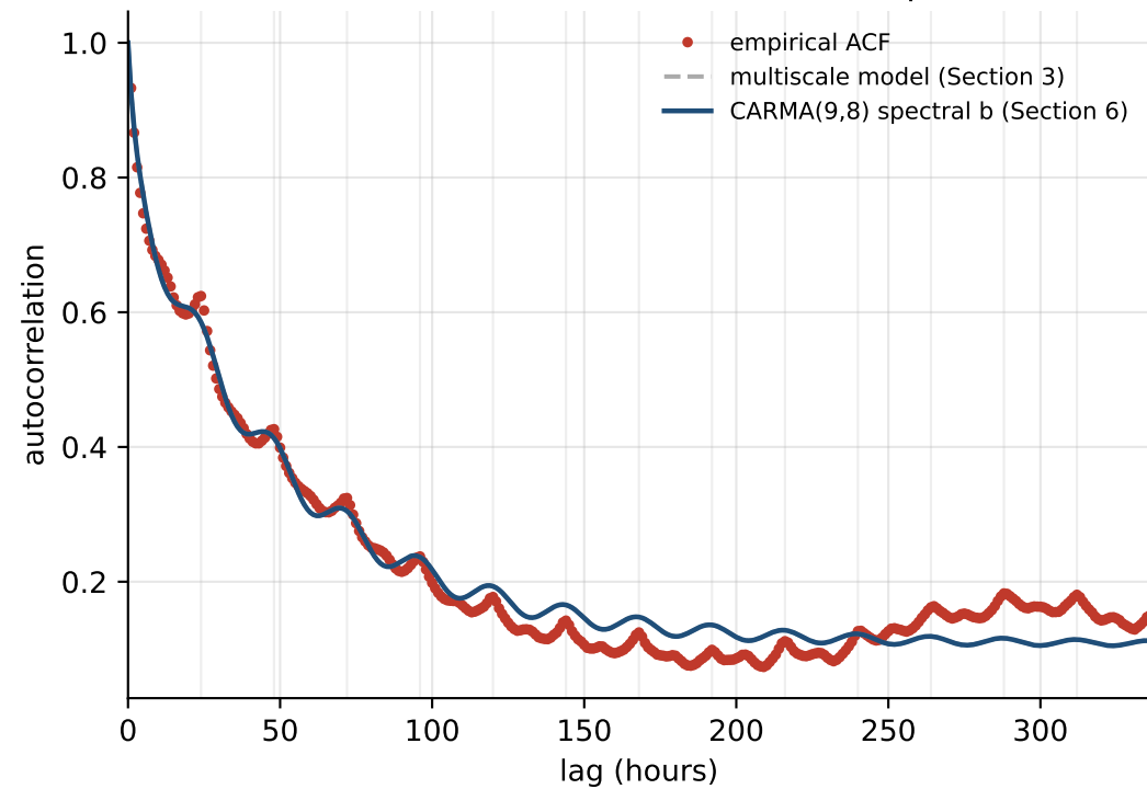
ACF: multiscale model vs CARMA(9,8) spectral b
