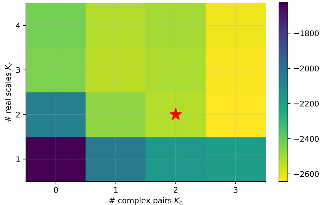
BIC (lower=better); \hat{a} \sim \dots = selected
