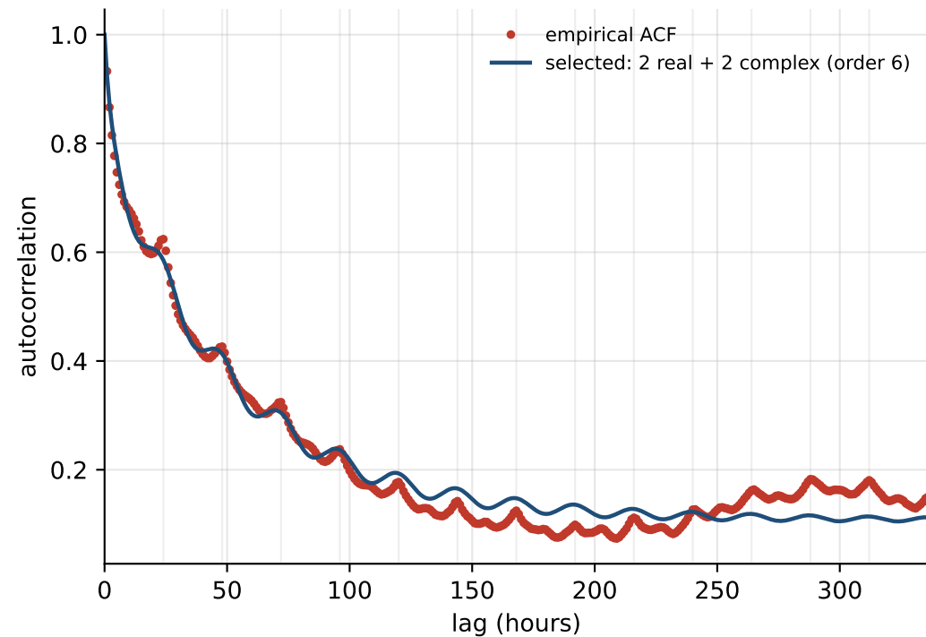
ACF fit at the selected order
