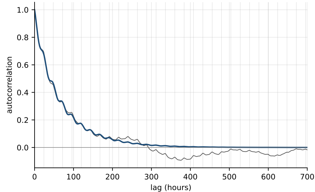
Multiscale ACF initialization
