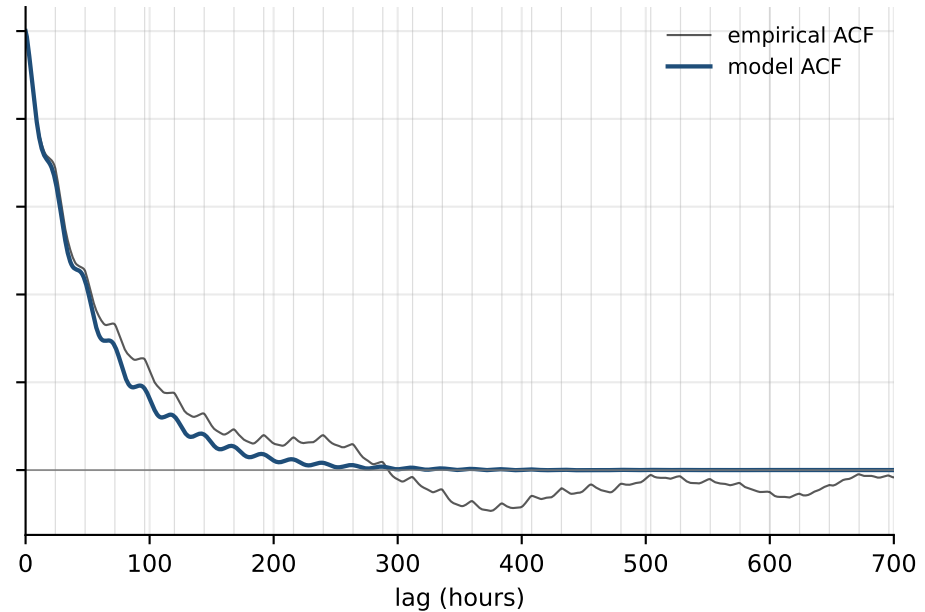
Final CARMA(4,3) QMLE ACF
