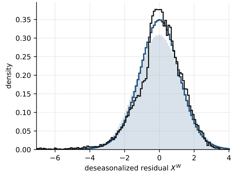
Residual factor
