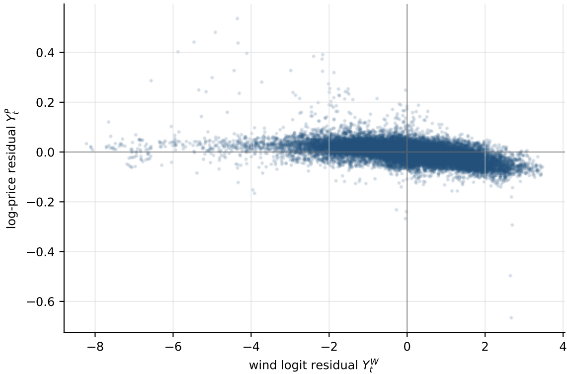
Raw residual levels, correlation = -0.4976
