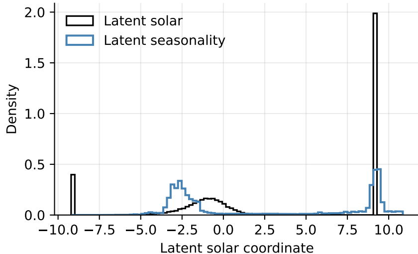
Latent distributions
