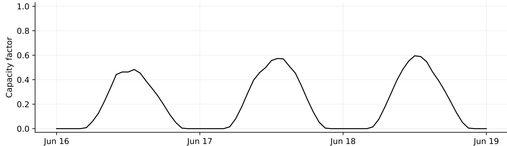
Raw solar capacity factor, three days in June 2025
