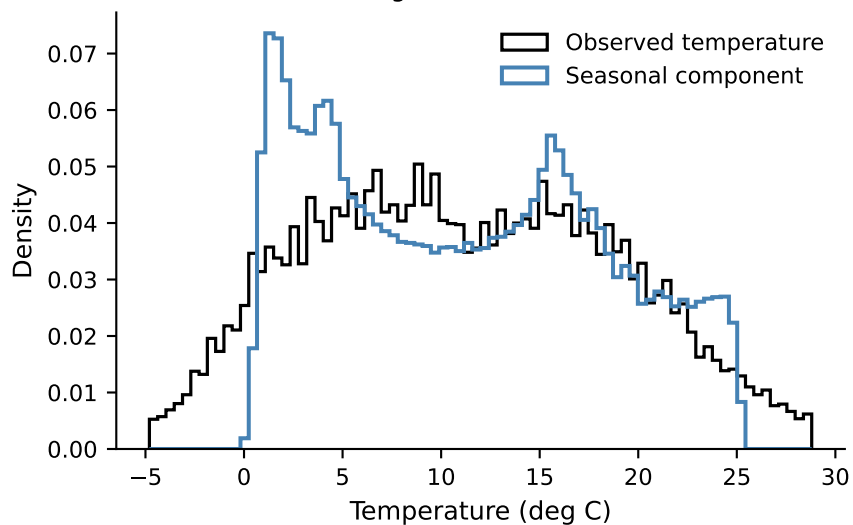
Marginal distributions
