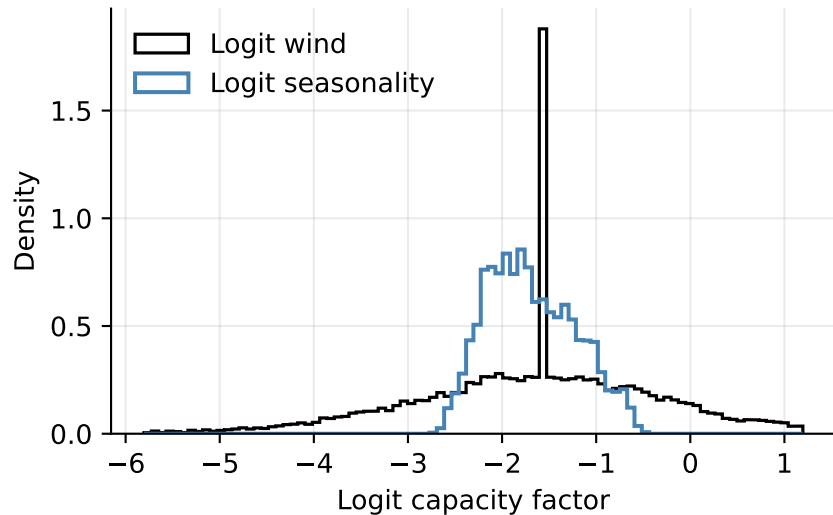
Latent distributions
