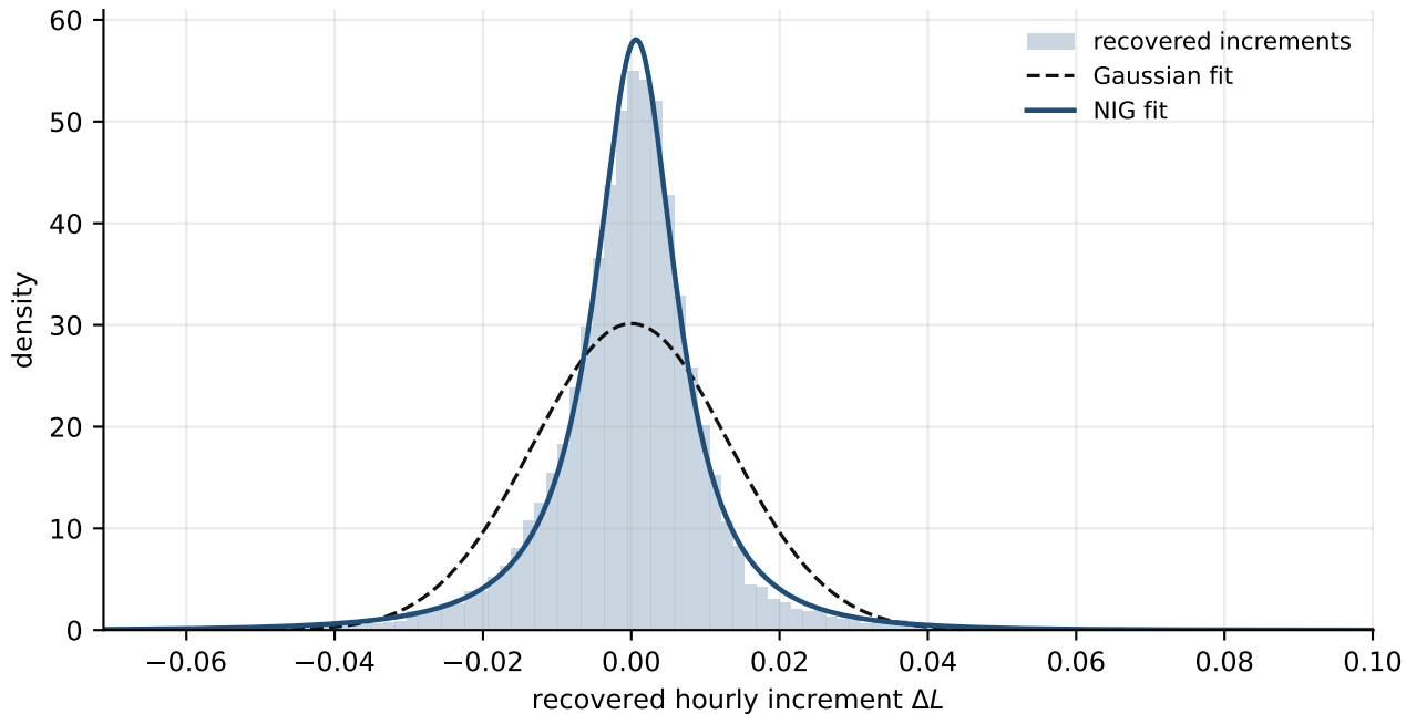
Recovered Levy driver distribution
