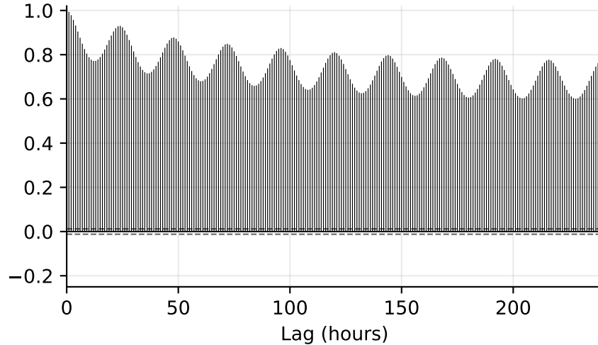
Observed temperature
