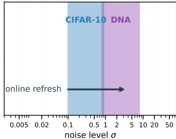
InfoNoise (data-adaptive)
